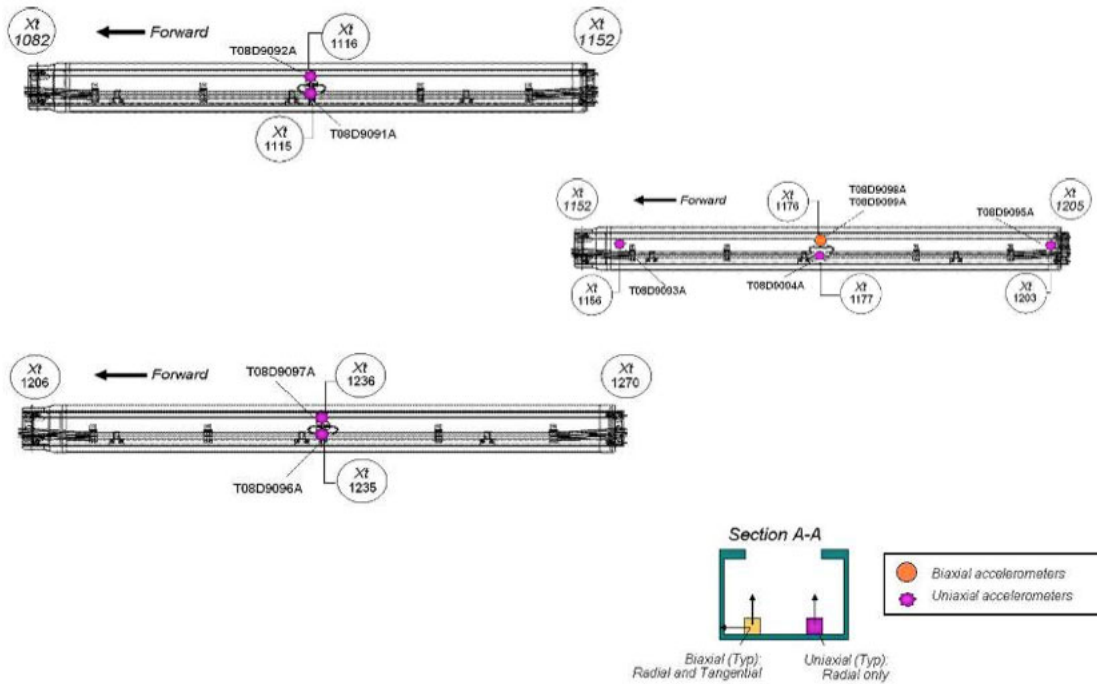
Figure 5.—Accelerometer Arrays in Three Segments of LH 2 Cable Tray (NTS).
