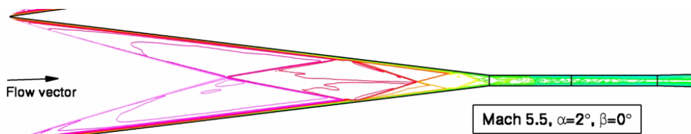
Figure 14. Mach 5.5, \alpha=2^\circ forebody and inlet shock pattern at the centerline.
