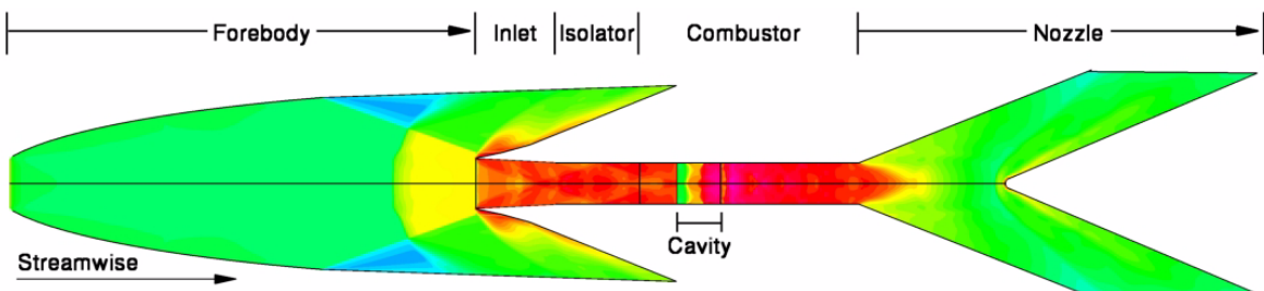
Figure 10. Flowpath surfaces — planform view.
