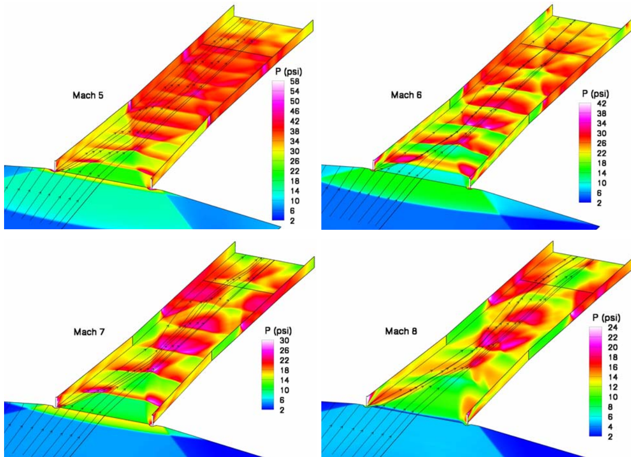
Figure 18. Inlet and isolator surface pressure at Mach 5, 6, 7, and 8 (no back pressure).
