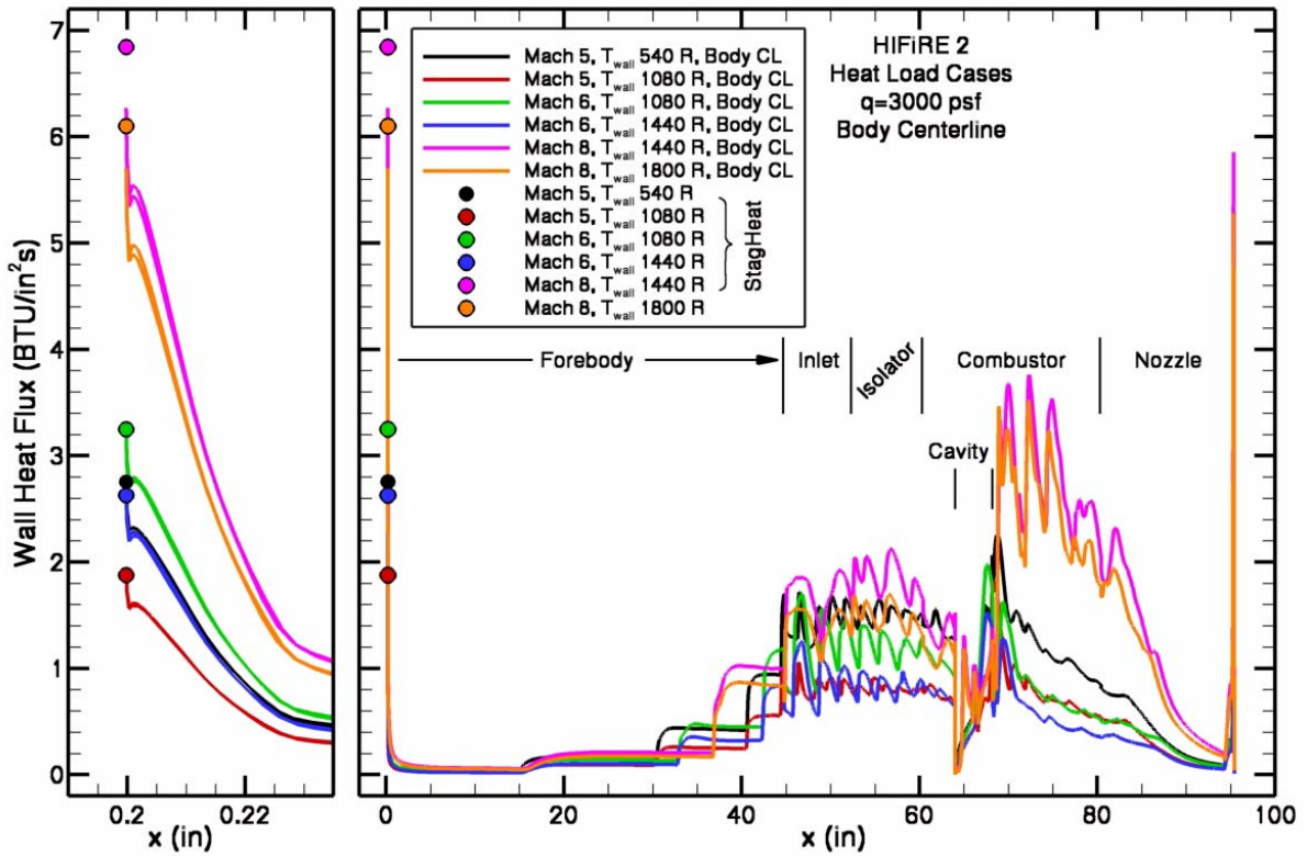
Figure 21. Flowpath centerline heat flux (no fuel injection).
