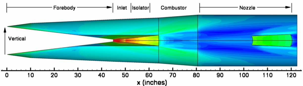
Figure 9. Side view.
