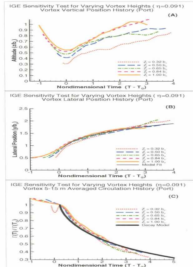
Figure 2. Sensitivity to vortex initiation height. Nondimensional height (a), nondimensional lateral position (b), and nondimensional 5-15 m averaged circulation (c) vs nondimensional time. "Decay model" in (C) from Eq.1 and "Curve fit" in (B) from Eq.2.
