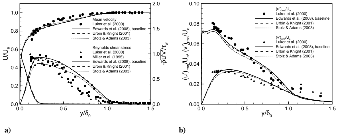
a) b) Figure 4. Effect of inflow method on (a) mean velocity profiles and Reynolds shear stress predictions, and (b) streamwise and wall-normal Reynolds stress predictions.
