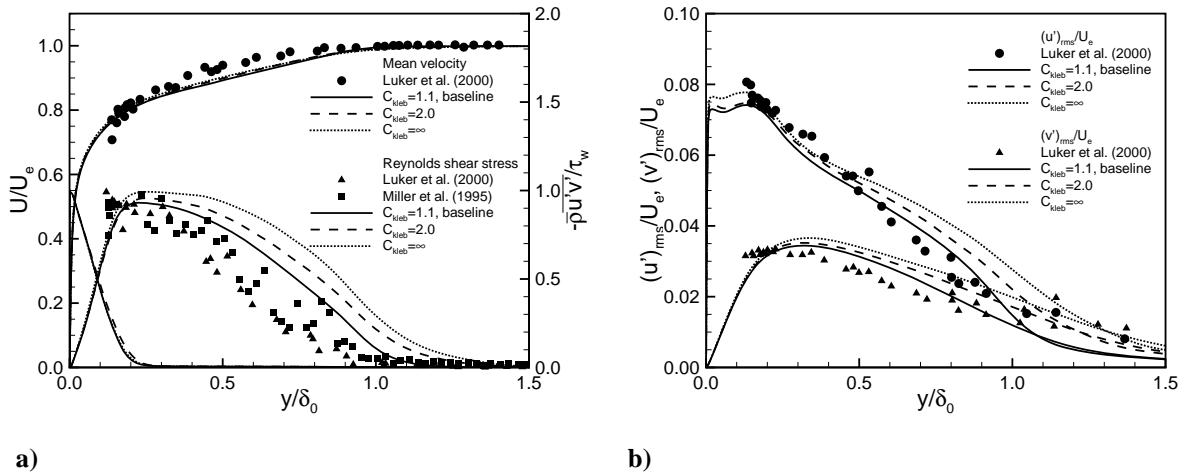
a) b) Figure 5. Effect of model constant C_{kleb} on (a) mean velocity profiles and Reynolds shear stress predictions, and (b) streamwise and wall-normal Reynolds stress predictions.
