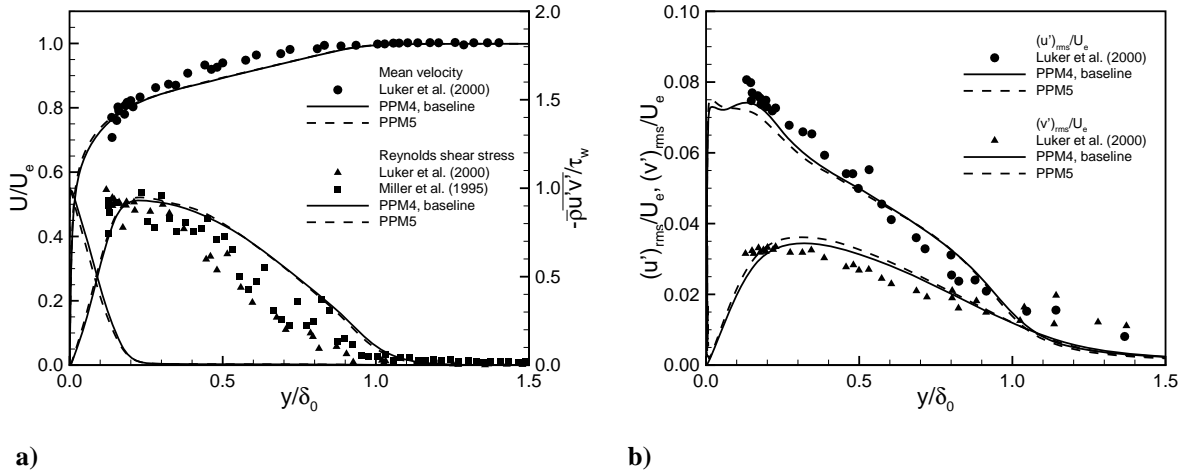
a) b) Figure 3. Effect of reconstruction method on (a) mean velocity profiles and Reynolds shear stress predictions, and (b) streamwise and wall-normal Reynolds stress predictions.
