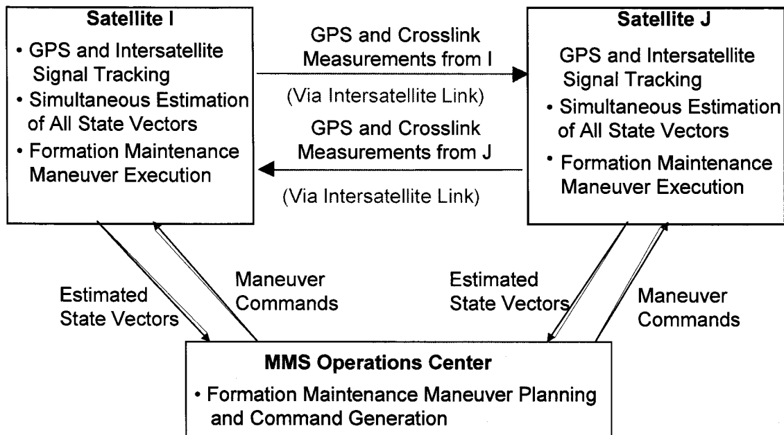
Figure 1: Space/Ground Navigation Configuration
