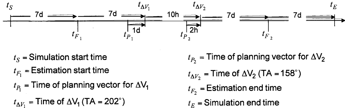
Figure 4: Simulation Timeline
