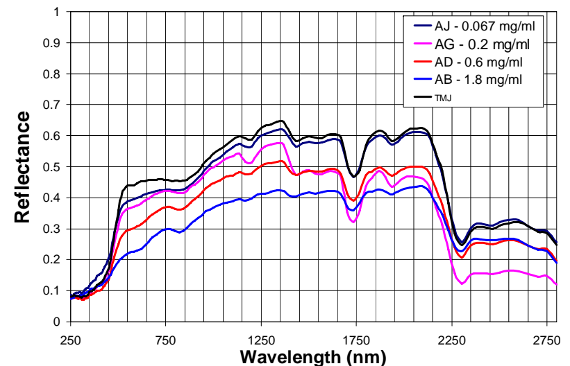
TMJ Coating With Varying Nanoshell Concentrations
