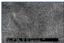
Nanofiltration
