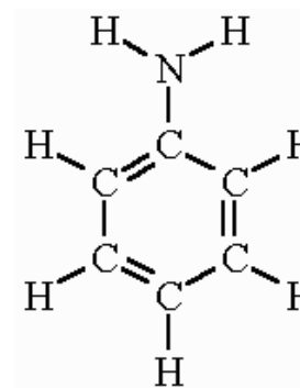
Aniline
