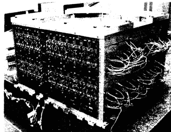
assembled single calorimeter module (1 of 16)
