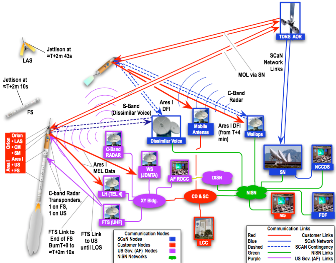
Figure 3. Launch/Ascent (Launch from T0 to ≈ T+6m 30s).
