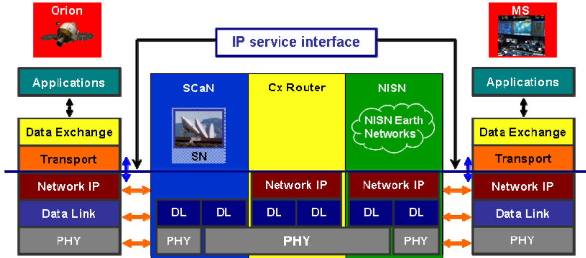
Figure 10. General End-to-End IP Network Architecture.
