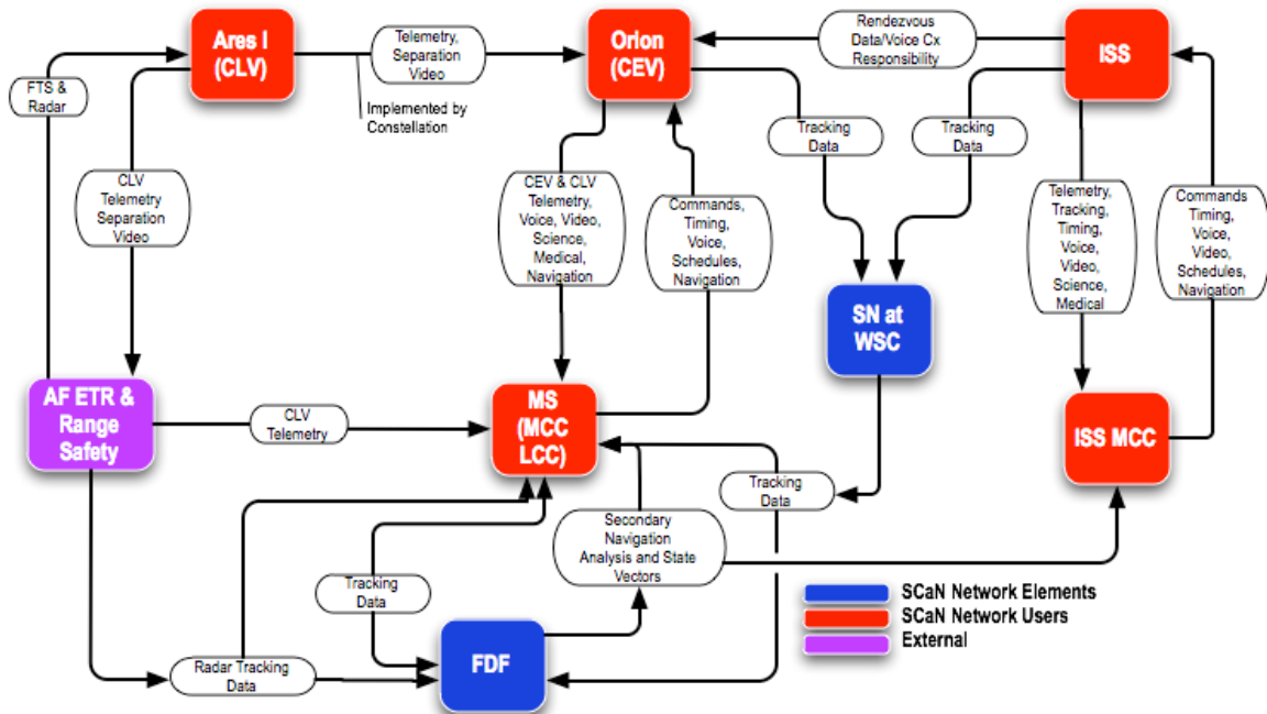
Figure 12. OV-2, Operational Information Exchange Diagram for the Orion-ISS Mission.
