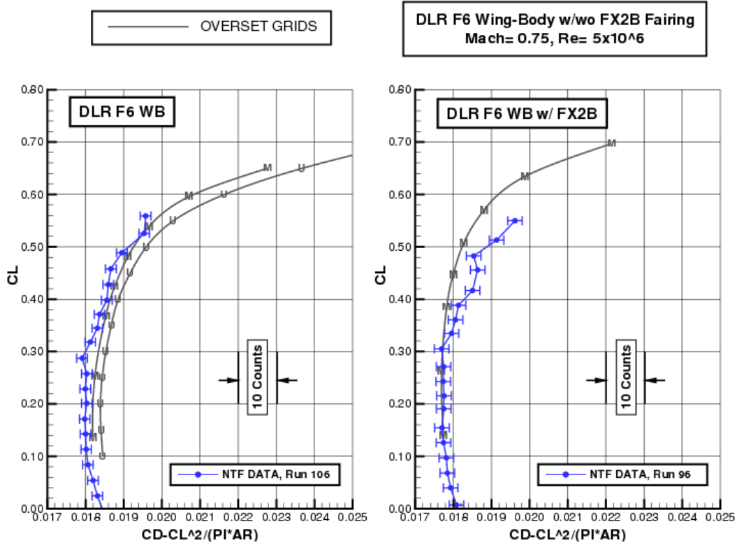
Figure 15. Case 1 Overset Mesh Idealized Profile Drag Polars.
