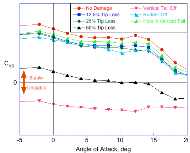
Figure 10. Vertical Tail Damage – Static Directional Stability
