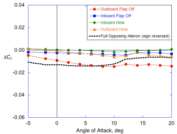
Figure 15. Wing Damage – Incremental Rolling Moment from Flap Loss or Hole
