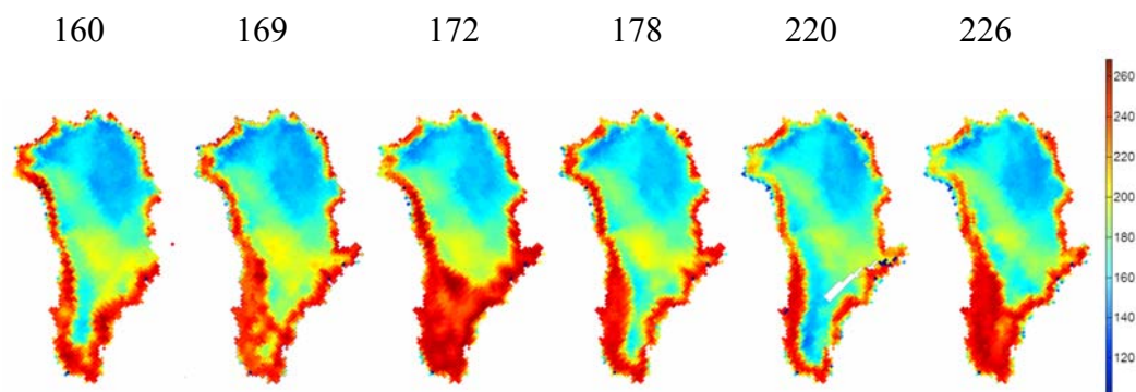
Figure 7. SSM/I brightness temperature over Greenland for 2004.
