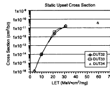
Figure 3: Error cross-sections observed in static upset.
