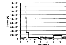
Figure 8: Power supply current during one exposure, with anomalous high current excursion. SEFI was detected after exposure.
