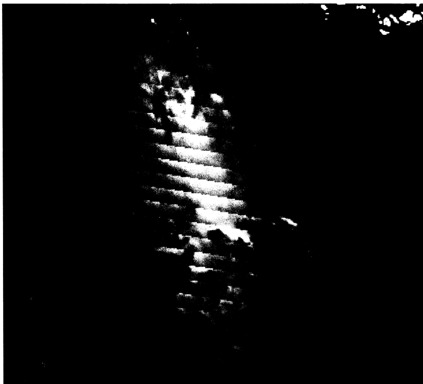
Figure 3. The effect of azimuth discontinuity. This is a zoom-in of a gridded RGB image of MODIS L1B top of the atmosphere reflectance, over Red sea, on day 136, 2005.
