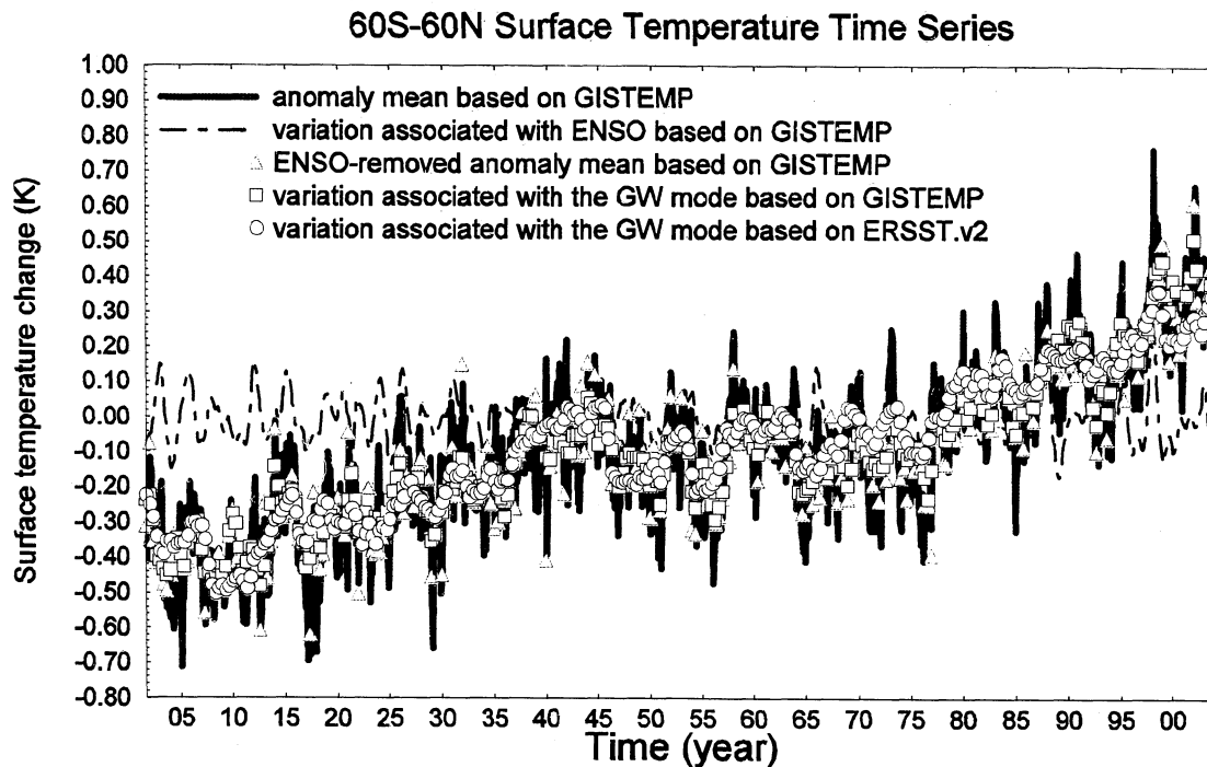
Figure 1. The time series of the GW trend in the 60°S-60°N latitude band. Because the 60°S-60°N zonal band covers 86.6% of the earth's surface and a reliable long-term observation record is lacking in the polar regions, the average temperature for this zonal band is assumed to roughly represent the known average temperature of the entire area of the earth.
