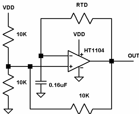
Fig. 1. Schematic of the temperature-to-frequency relaxation oscillator circuit.
