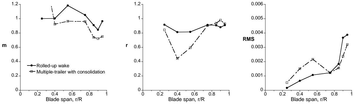
Fig. 29: Slope, correlation coefficient, and RMS error values for H-34 at \mu = 0.129 ; harmonics 3-10
