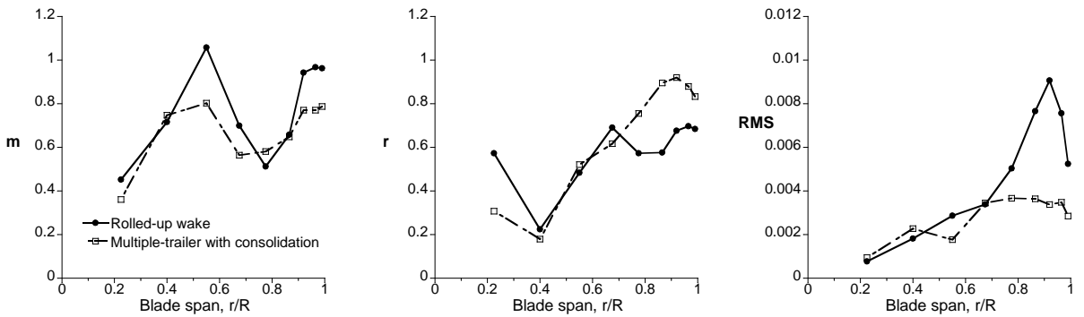
Fig. 30: Slope, correlation coefficient, and RMS error values for UH-60A at \mu = 0.149 ; harmonics 3-10
