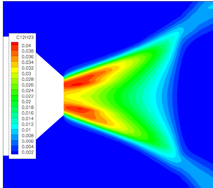
Figure 20.—Contours of fuel mass fraction ( C_{12}H_{23} ) in an axial slice at the Y=0 mm mid-plane.
