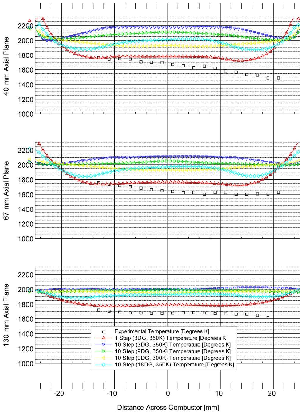
Figure 13.—Comparison of temperature versus spanwise distance in the axial Y-Z plane with Z = 0 mm.
