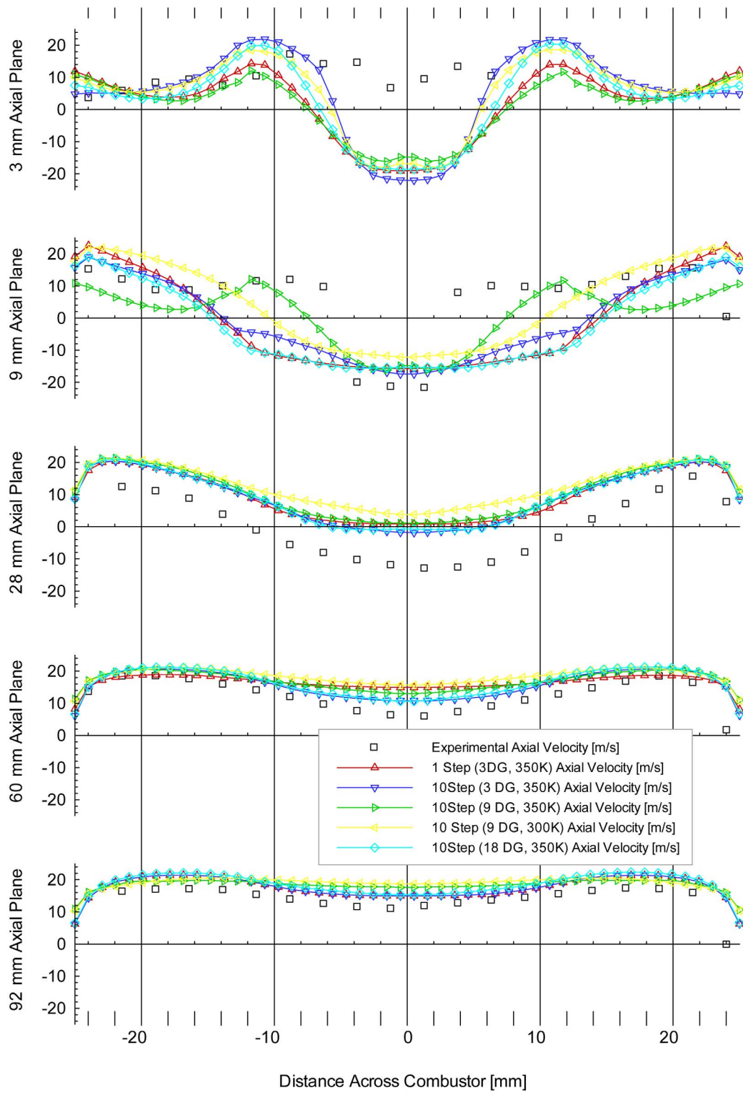
Figure 8.—Comparison of axial velocity versus spanwise distance in the axial Y-Z plane with Z = 0 mm.
