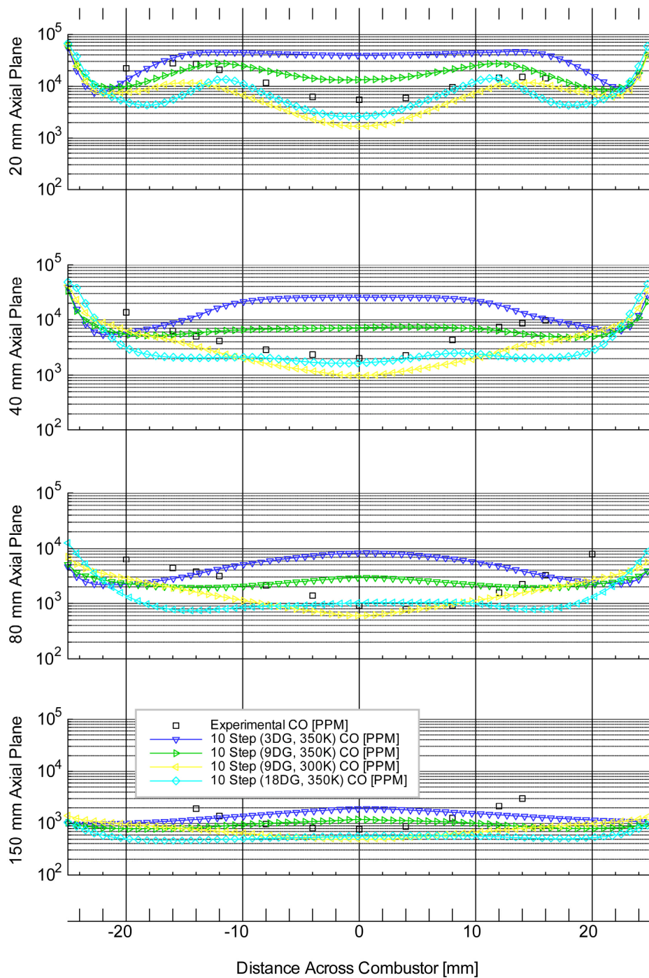
Figure 15.—Comparison of carbon monoxide amounts versus spanwise distance in the axial Y-Z plane with Z = 0 mm.
