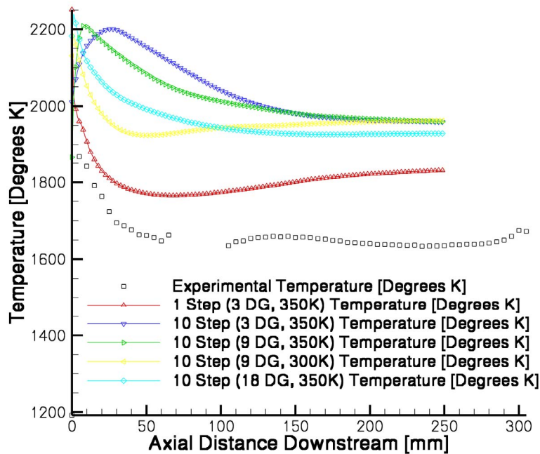
Figure 11.—Comparison of temperature versus axial distance at the centerline.
