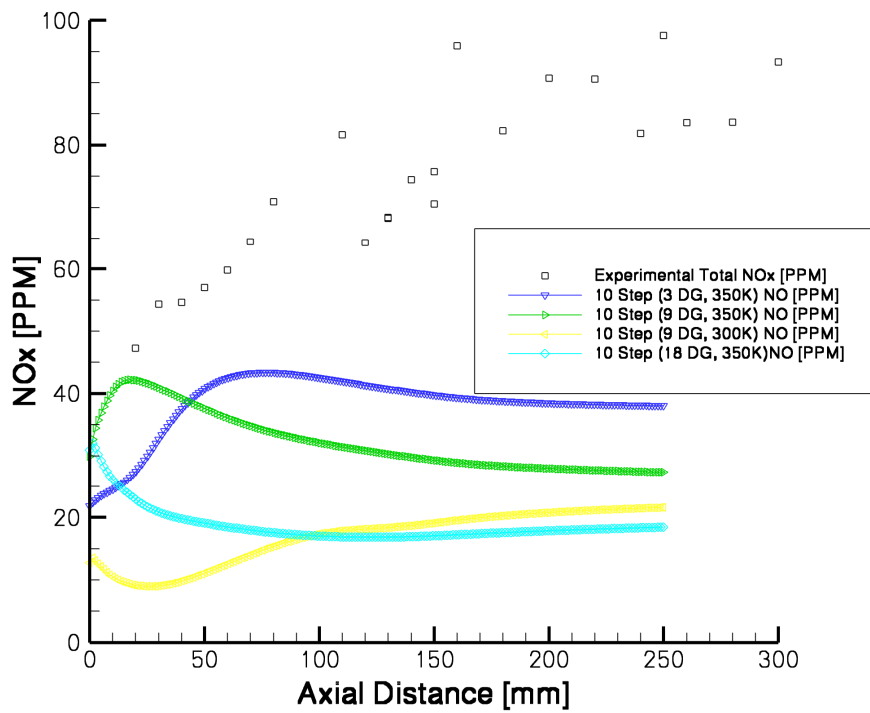
Figure 16.—Comparison of nitrogen oxides amount versus axial distance at the centerline.
