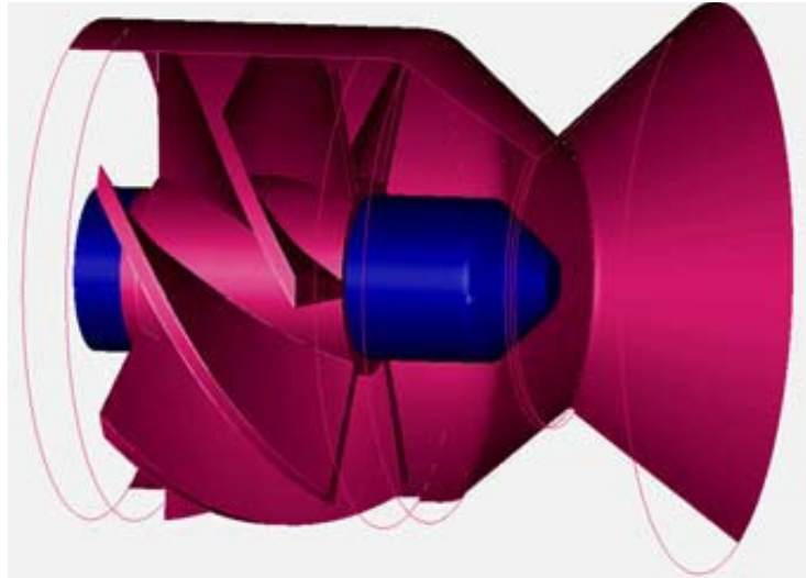
Figure 1.—Single element LDI injector geometry.
