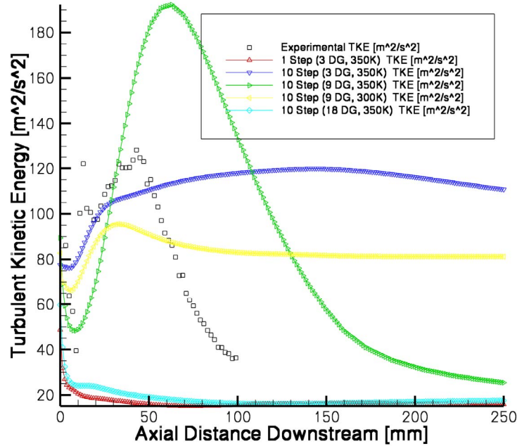
Figure 10.—Comparison of turbulent kinetic energy versus axial distance at the centerline.
