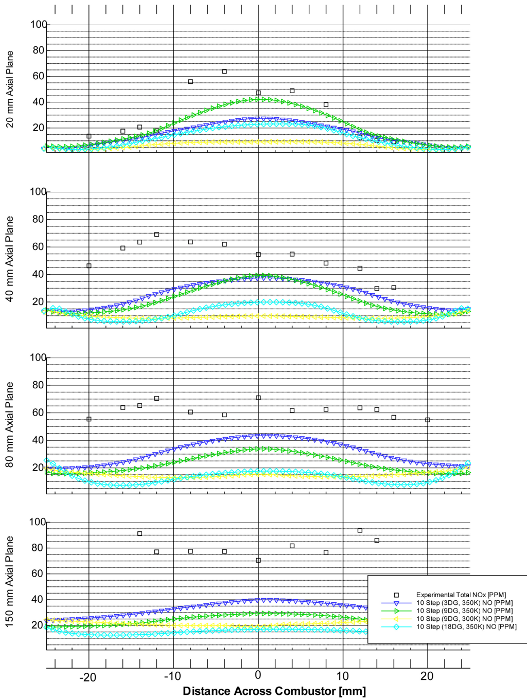
Figure 17.—Comparison of nitrogen oxides amount versus spanwise distance in the axial Y-Z plane with Z = 0 mm.
