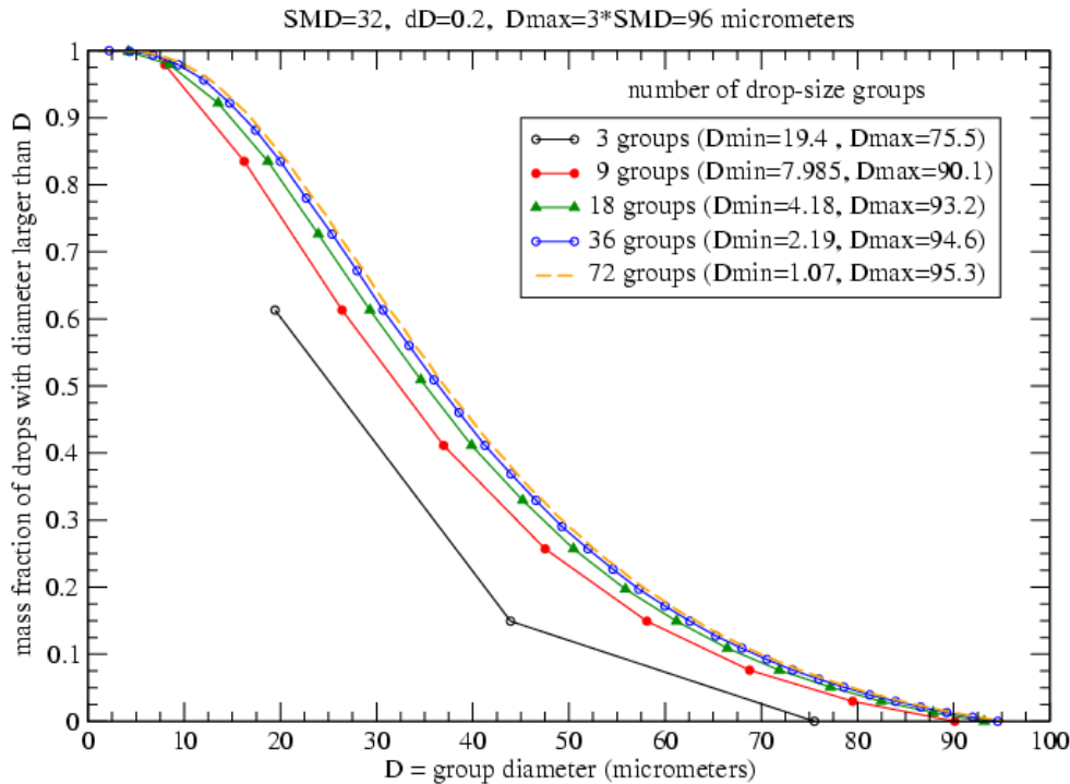
Figure 3.—Cumulative drop size distribution (spray initial condition).
