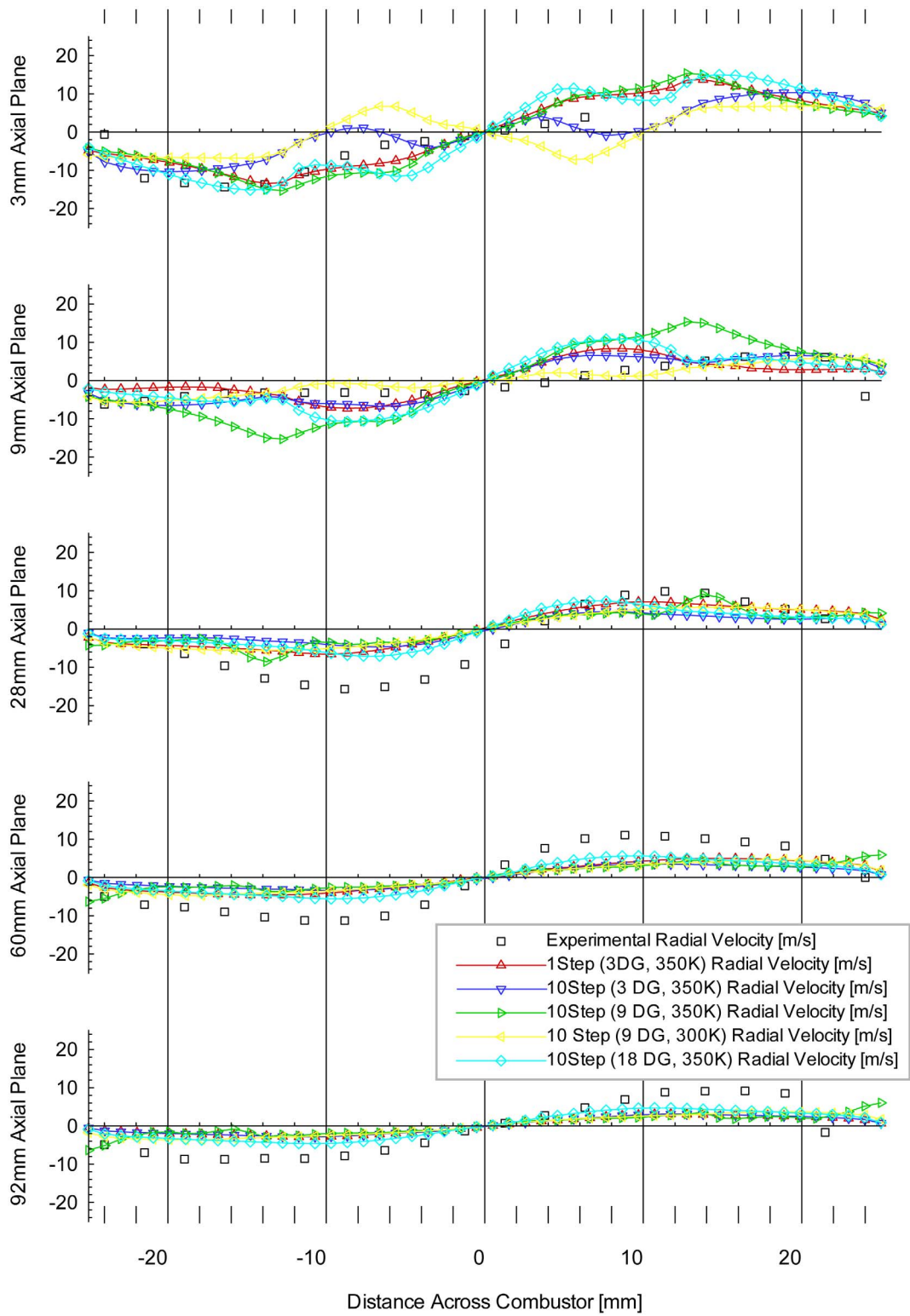
Figure 9.—Comparison of radial velocity versus spanwise distance in the axial Y-Z plane with Z = 0 mm.
