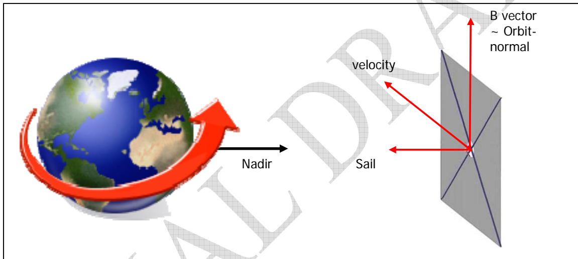
Figure 8: Orbit Geometry
