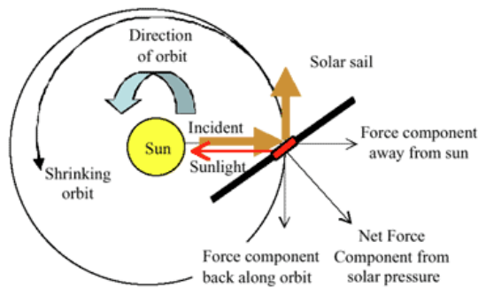
Figure 1: Solar Radiation Thrust Force (NASA/JPL)
