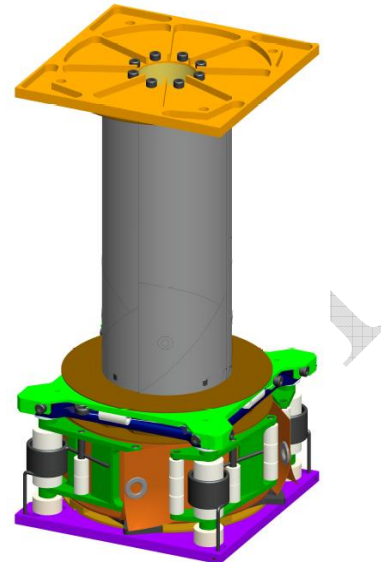
Figure 4: Sail Subsystem
