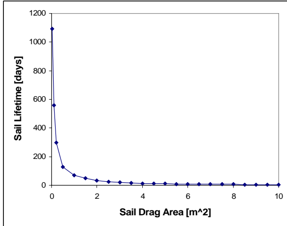
Figure 7: Mission Duration as a Function of Sail Size
