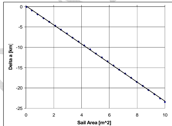
Figure 6: Orbit Decay as a Function of Sail Area within a 24 hour time frame
