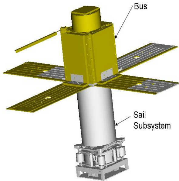
Figure 3: Panel Deployed Configuration
