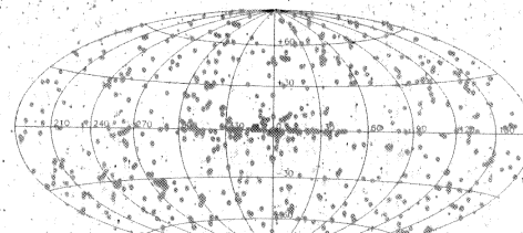
Fig. 3. Sightlines for which IXO will be able to determine abundances of silicate-forming elements to better than 20%.
