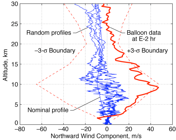
Figure 6. Northward wind component variation from GRAM-95 model.
