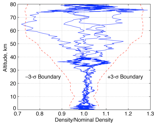
Figure 5. Density variation from GRAM-95 model.
