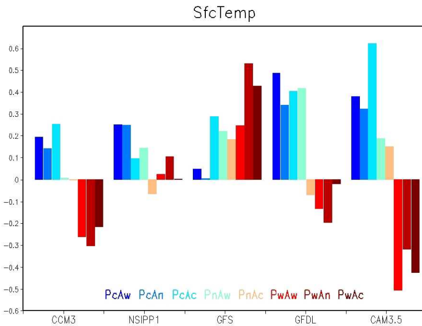
Figure 8: The annual and continental United States mean responses for a) precipitation and b) surface temperature for all 8 combinations of the Pacific and Atlantic patterns for the 5 AGCMs (see Table 1).
