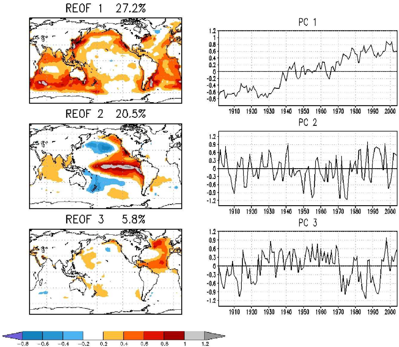
Figure 1: The three leading rotated EOFs (left panels) and associated PCs (right panels) of the annual mean SST based on the period 1901-2004. The values are scaled so that the product of the PCs and EOFs gives units of ^{\circ}\text{C} . The Pacific and Atlantic patterns reflect the two standard deviation forcing amplitude applied to the models, while the trend pattern must be divided by a factor of two to obtain the forcing amplitude.
