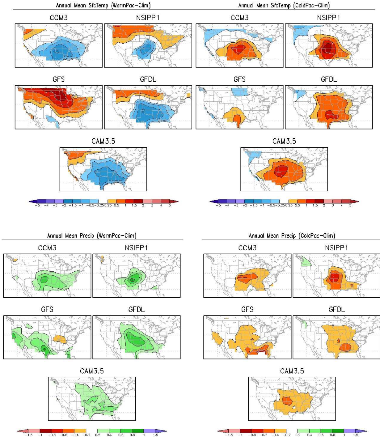
Figure 6: Annual mean surface temperature (top panels, units: ^{\circ}\text{C}/\text{day} ) and precipitation (bottom panels, units: \text{mm}/\text{day} ) responses to the PwAn (left panels) and PcAn (right panels) SST anomaly pattern. The anomalies for each model are computed with respect to its annual mean response to a simulation in which the model is forced with climatological SSTs. See text for details on the SST forcing.
