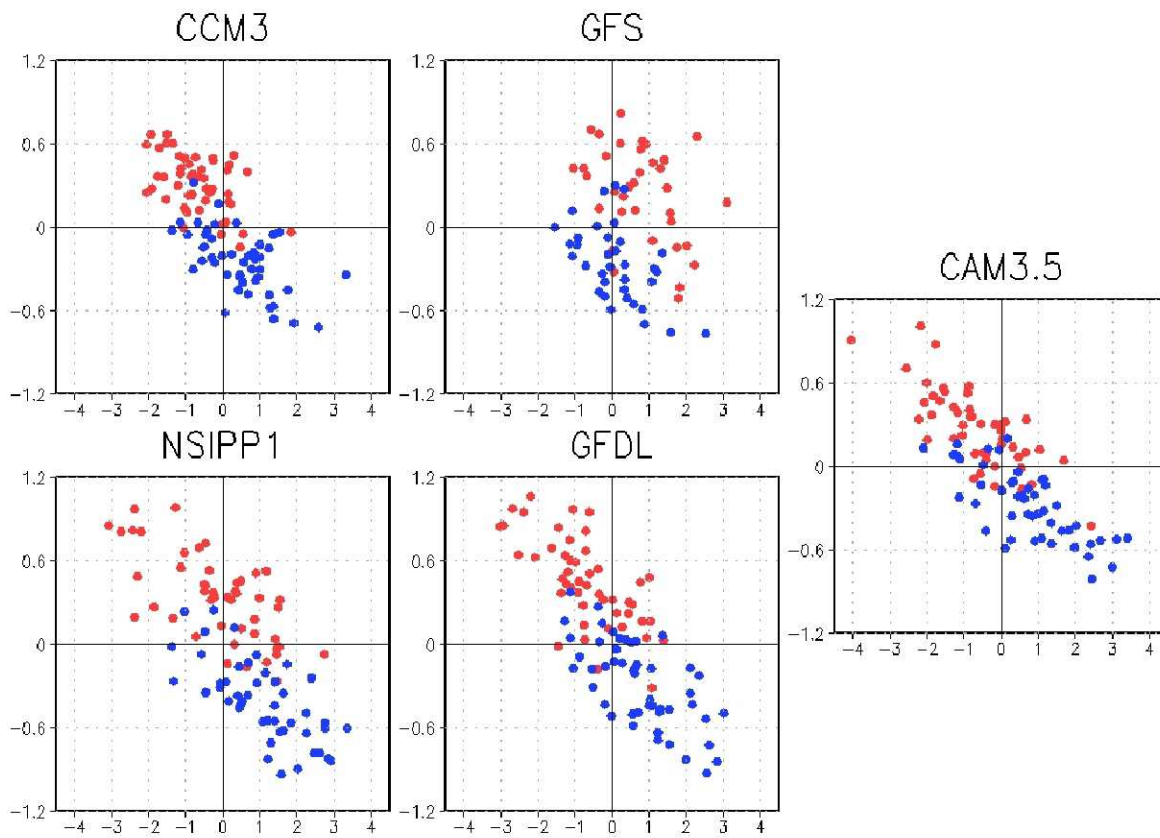
Figure 7: Scatter plots of the Great Plains annual mean precipitation (ordinate) versus surface temperature (abscissa) response to the PwAn (red dots) and PcAn (blue dots) SST anomaly patterns for the Great Plains area average. Each point represents one of 50 (35 for the GFS model) years of each run.
