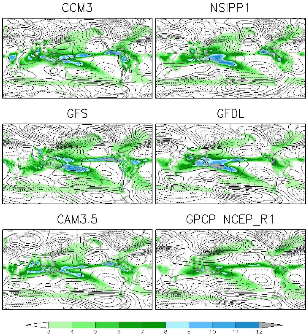
Figure 2: Annual mean precipitation and 200mb eddy height field averaged over the years 1980-1998. The model results are from AMIP-style runs from each model (runs forced by observed SSTs). For the observations (lower right panel), the precipitation is from GPCP (Adler et al. 2003) and the height fields are from the NCEP/NCAR reanalyses (Kalnay et al. 1996). The time period was chosen in order to have a common set of years for each model. Contour interval for the height field is 20m (negative values are dashed and the zero line is the first solid contour). Precipitation is in mm/day.
