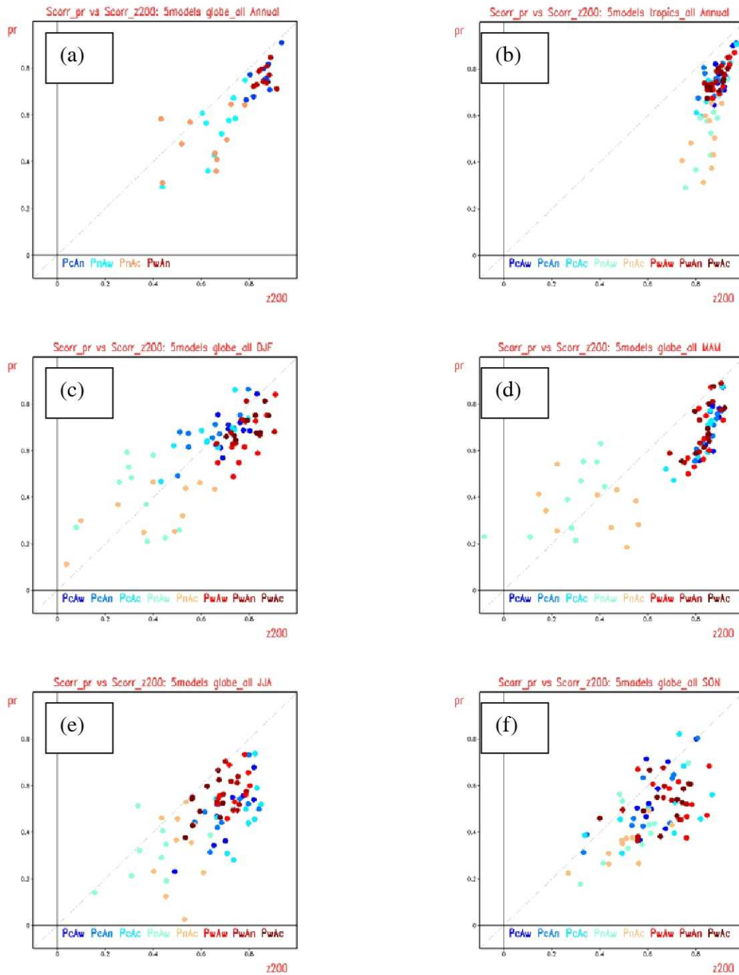
Figure 3: Spatial correlations of precipitation anomalies (ordinate) versus spatial correlations of 200mb height anomalies (abscissa) for the various combinations of models and for the various combinations of the Pacific and Atlantic forcing patterns. a) global correlations of annual means limited here to the 4 individual Pacific and Atlantic forcing patterns. b) tropical correlations ( \pm 30^\circ latitude) of annual means, c) global correlations for DJF d) global correlations for MAM, e) global correlations for JJA, and f) global correlations for SON. See text for details. The colors refer to the forcing patterns indicated along the bottom of the plots.
