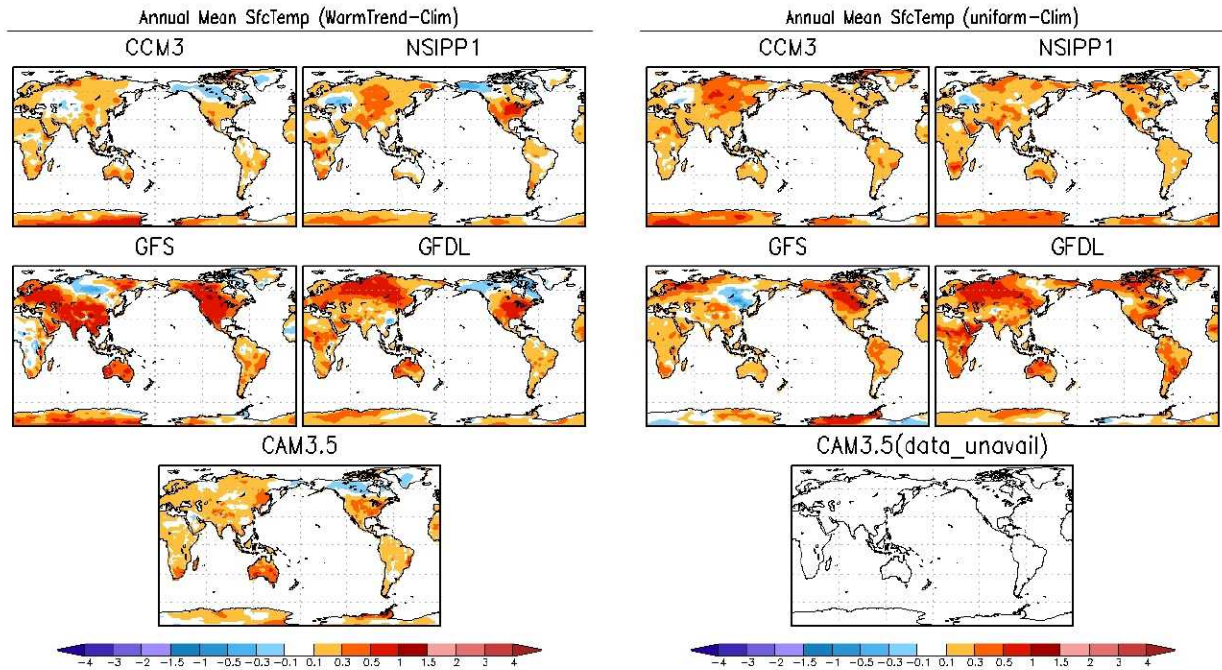
Figure 12: Left panels: The annual mean surface temperature response to the positive phase of the trend pattern. Right panels: The annual mean surface temperature response to a globally uniform SST warming of 0.16 °C. The uniform warming run was not performed with CAM3.5. Units: °C.
