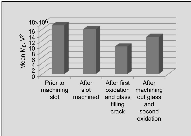
Figure 8.—Ultrasonic guided wave (mean total energy M_0 ) results on sample RCC1 (Fig. 2). Measurement variability is about 2 percent based on repeated trials.
