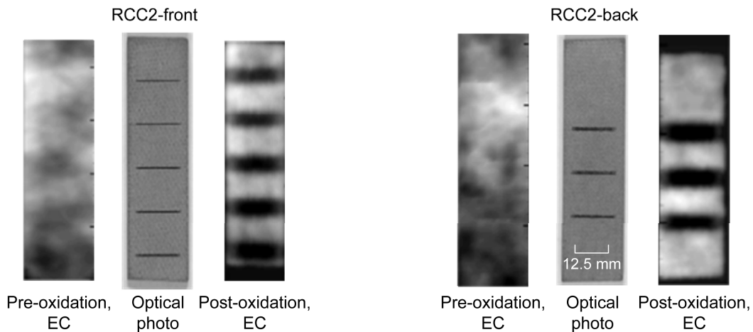
Figure 6.—Eddy current (EC) results.
