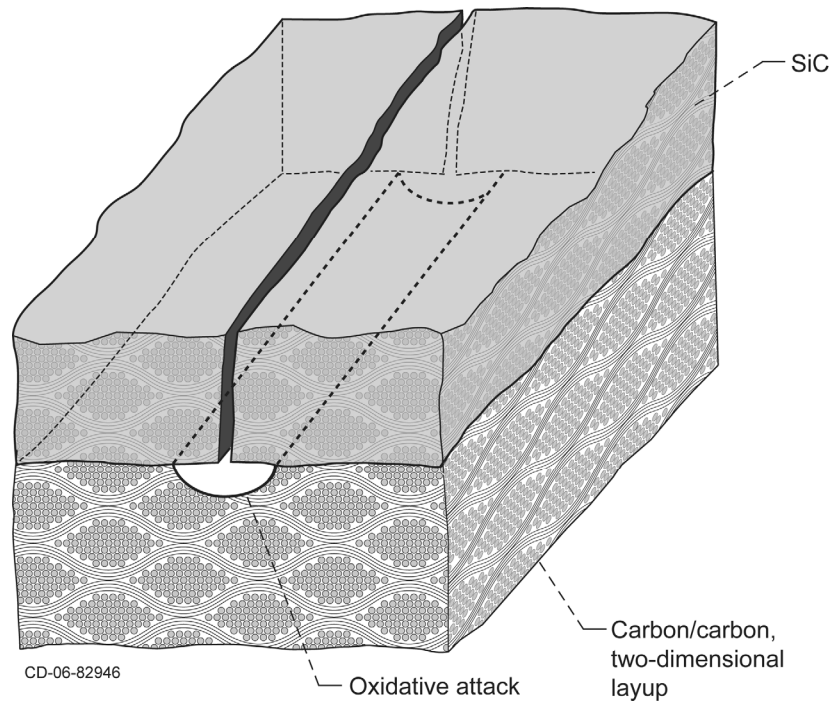
Figure 1.—Schematic of SiC-protected carbon/carbon used in this study.
