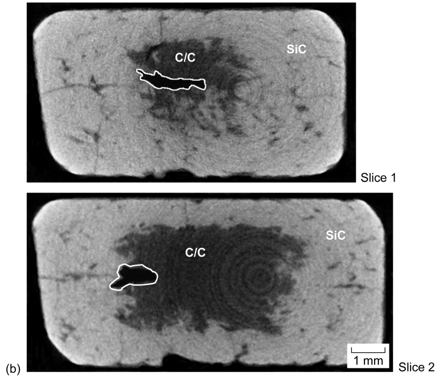
Figure 10.—X-ray CT of SiC-coated RCC oxidized for 2.5 hr in air at 1143 °C. (a) Location of CT slices. (b) Two CT slices.
