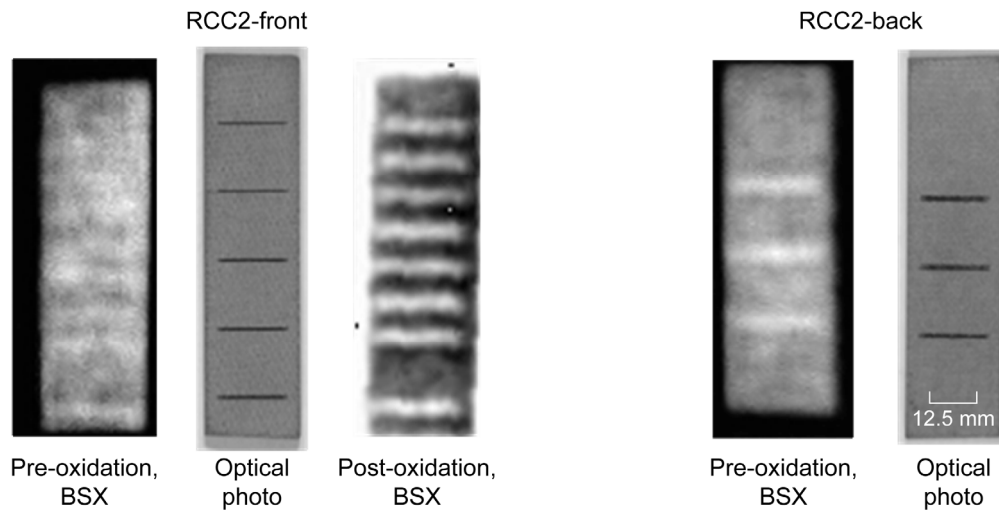
Figure 5.—Backscatter x-ray (BSX) results.
