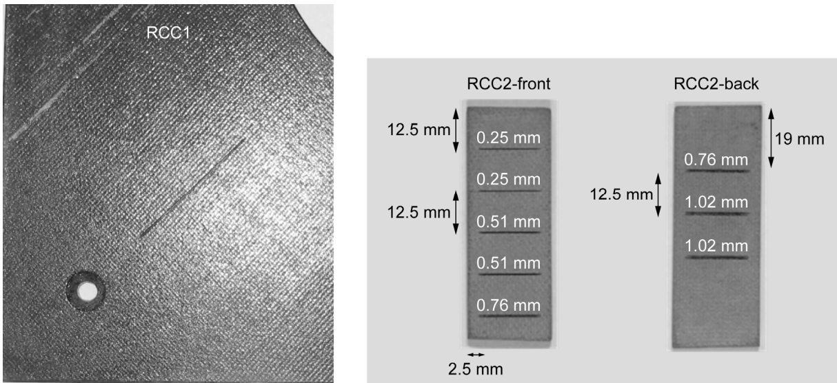
Figure 2.—Photographs of machined RCC samples with machined slots. Nominal widths of slots are shown above the slot and spacing between slots and from edges is also shown.
