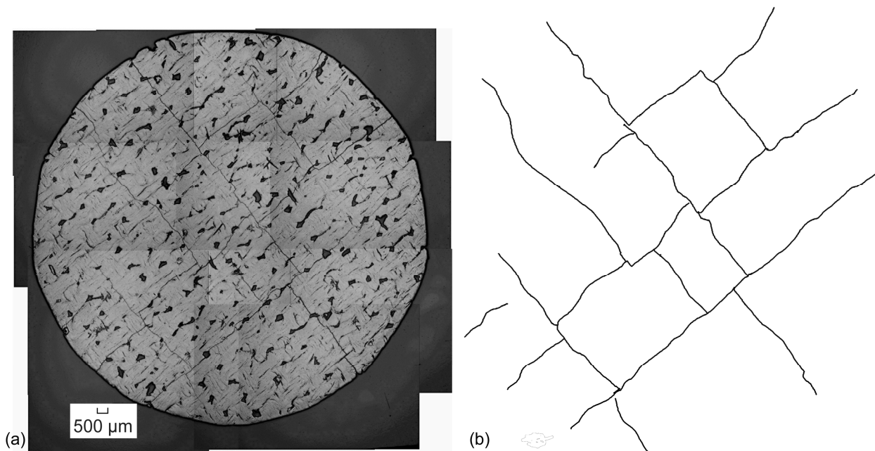
Figure 3(a).—RCC disk with craze crack pattern on the surface. (b) 'Skeleton' trace of crack pattern.
