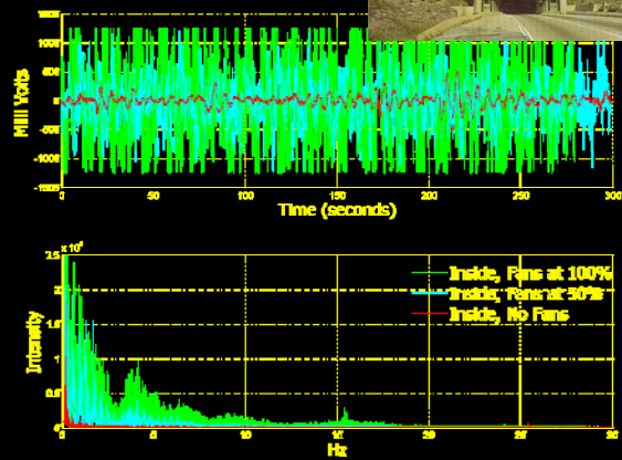
Figure 12: Infrasonic Measurement Inside the tunnel
