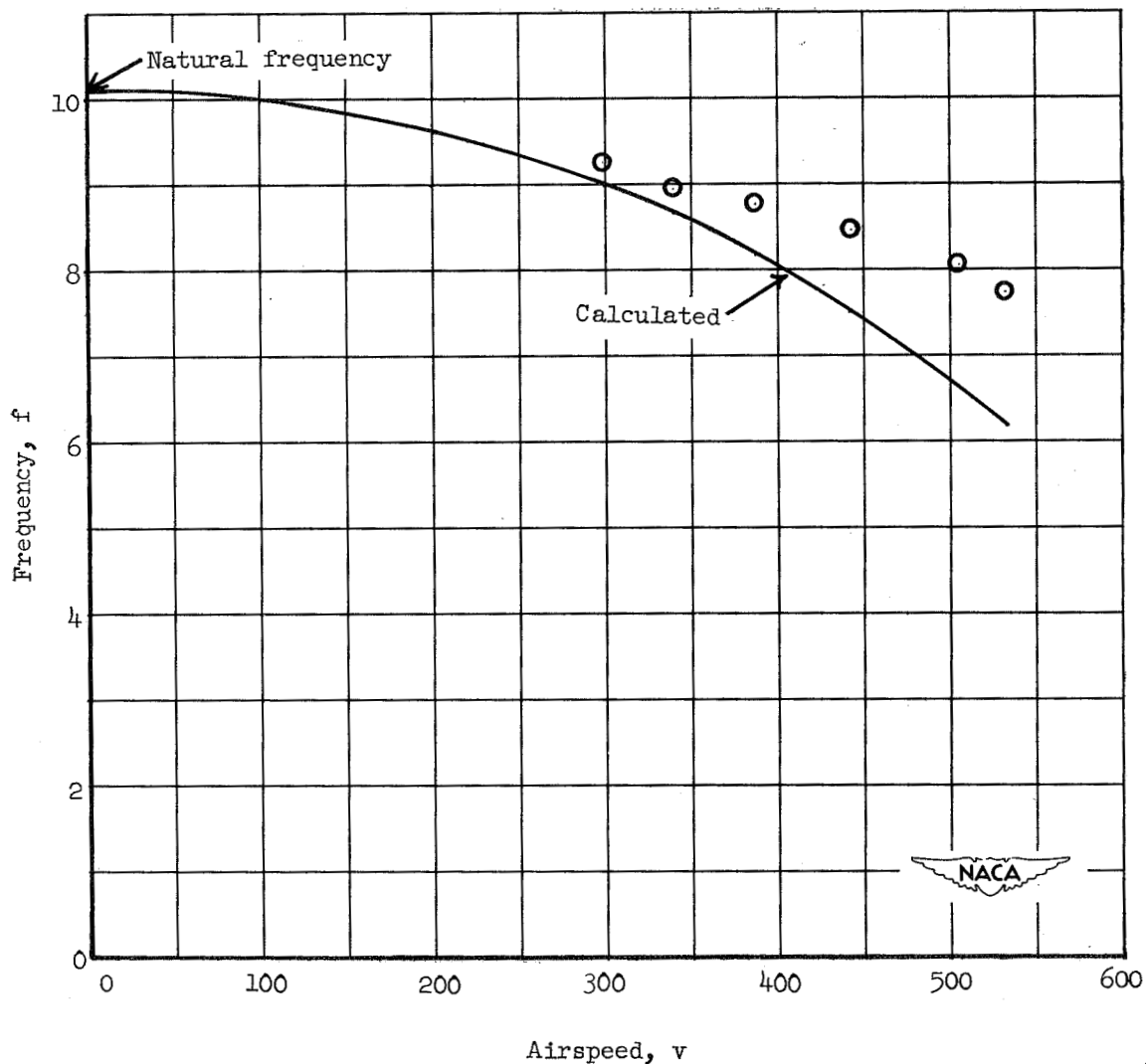
Figure 4.- Plot of frequency of yawing oscillations against airspeed for the airfoil-shaped body. (Table 3, test series II.)
