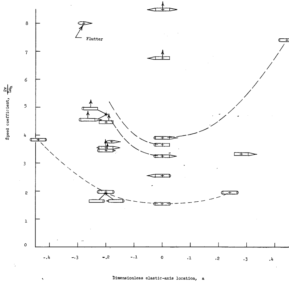
(a) Speed coefficients at onset of yawing oscillations. (b) Frequency ratios at onset of yawing oscillations.
