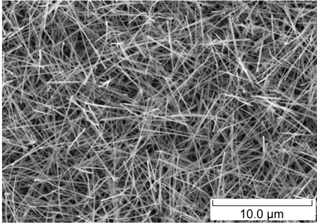
Figure 7.—SEM image of TiO 2 nanowires as grown upon Ti foil using the controlled oxidation method.
