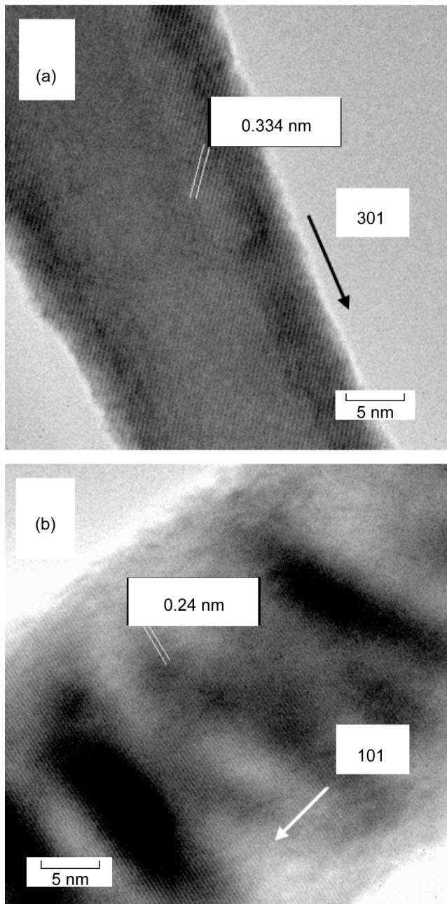
Figure 5.—HRTEM image. (a) A single-crystal SnO 2 nanowire, VLS mechanism. (b) A single-crystal SnO 2 nanowire versus mechanism.
