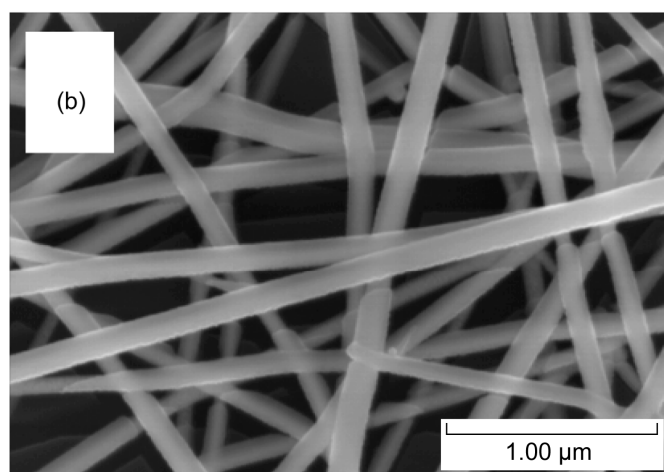
Figure 11.—SEM image of calcined SnO 2 nanofibers.
