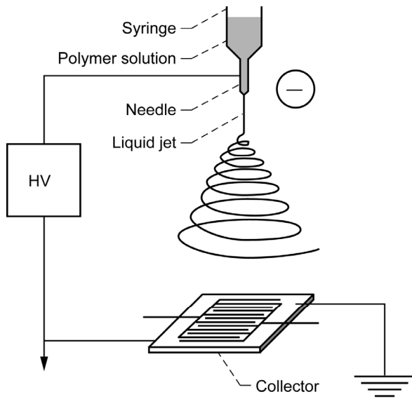
Figure 3.—Schematic of the experimental setup for electrospinning synthesis of nanofibers.
