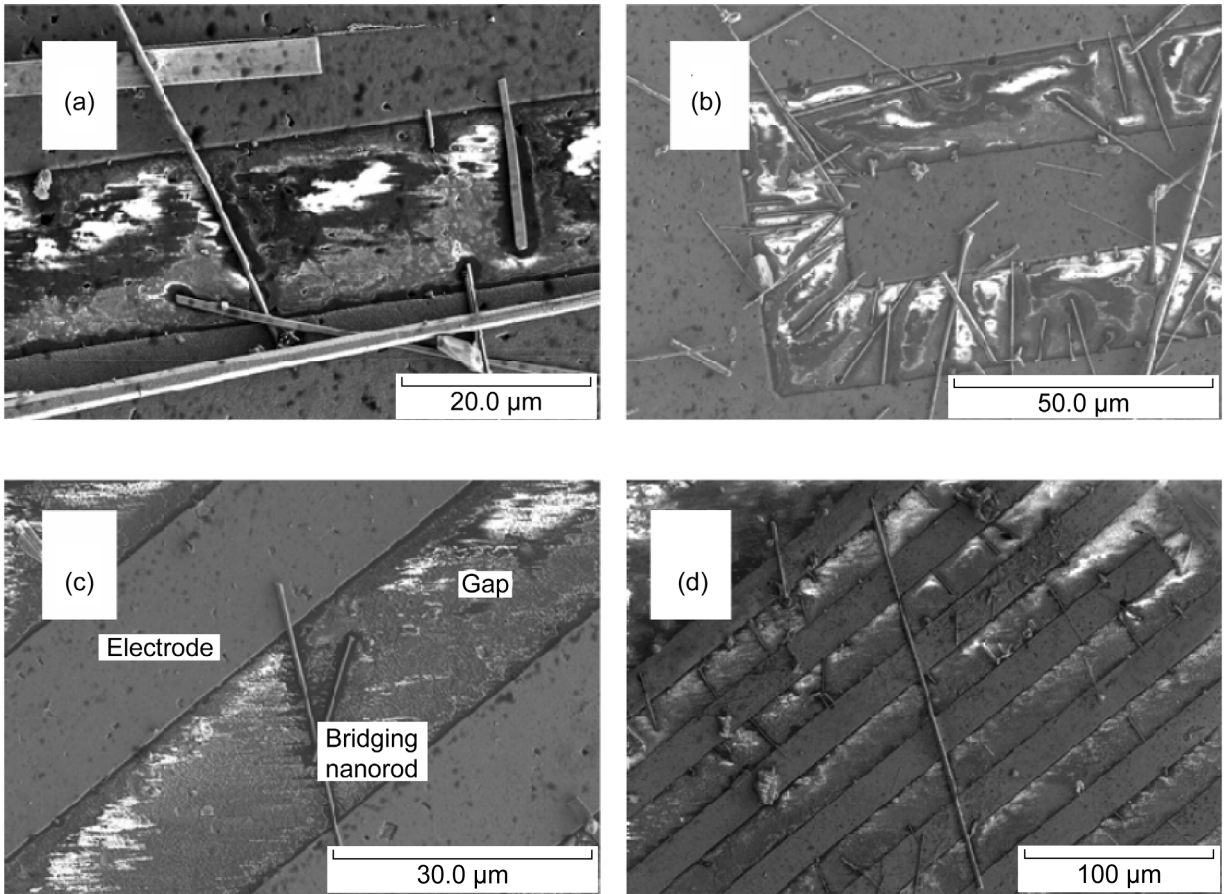
Figure 14.—Contact deficits include (a) and (b) failure to bridge and multiple junction contacts between nanowires. (c) Suspended nanowires. (d) Multiple bridging by a single nanowire.
