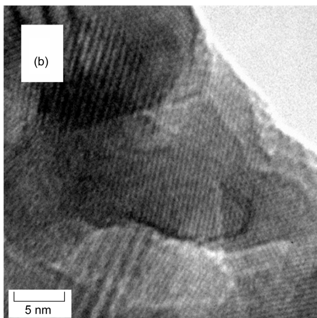
Figure 12.—HRTEM image of calcined nanofibers. (a) Lower resolution. (b) Higher resolution.
