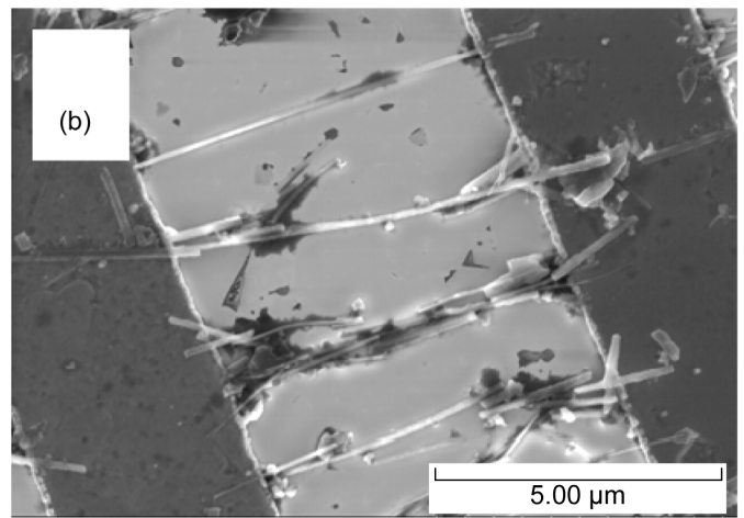
Figure 17.—SEM images illustrating more homogeneous dispersion and alignment by E-field induced torque in concert with dielectrophoresis. Purification aids the uniformity of the deposited material.
