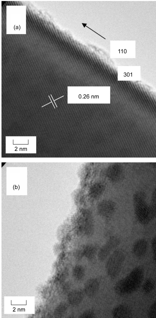
Figure 18.—HRTEM image of Pd deposited on \text{SnO}_2 nanowires. As illustrated the catalyst particles are relatively uniform in size and shape. The very high magnification image shows the single-crystal structure of the deposited catalyst.
