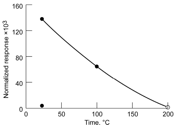
Figure 25.—SnO 2 nanowire sensor response versus temperature, filled circles are with Pd catalyst, nonfilled circles are without catalyst.
