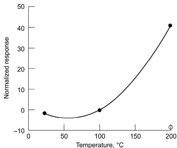
Figure 23.—TiO 2 nanowire sensor response versus temperature, filled circles are with Pt catalyst, nonfilled circles are without catalyst.
