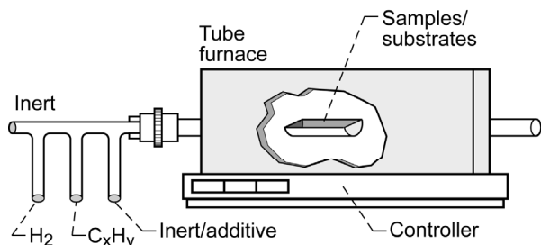
Figure 2.—Schematic of the experimental setup for TEC synthesis of nanowires.
