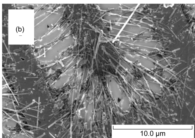
Figure 16.—SEM image illustrating concentrated collection of TiO 2 nanowires by dielectrophoresis, acting preferentially in the region of highest E-field gradient.
