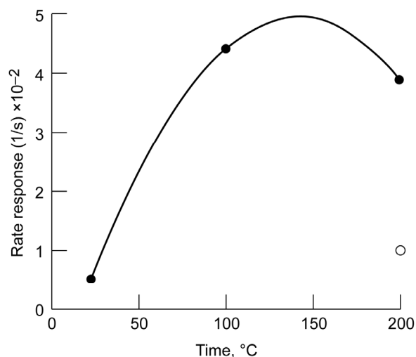
Figure 26.—SnO 2 nanowire sensor response rate versus temperature, filled circles are with Pd catalyst, nonfilled circles are without catalyst.
