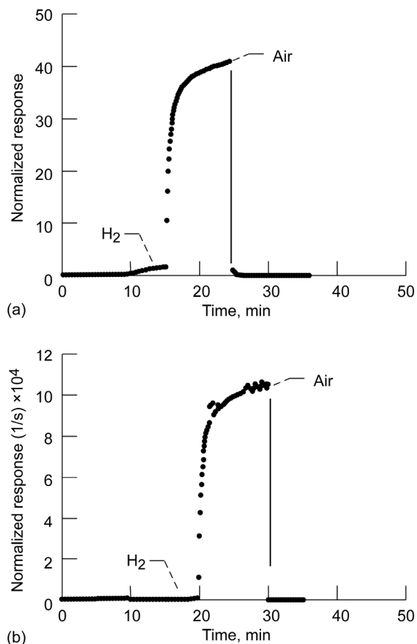
Figure 27.—(a) TiO_2 nanowire with Pt catalyst. (b) SnO_2 with Pt catalyst.
