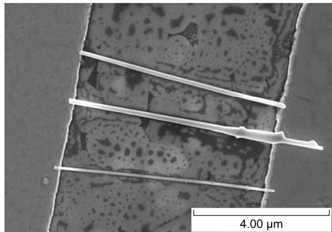
Figure 15.—Ideal characteristics are illustrated by the bridging of single nanowires and parallel alignment with each nanowire forming individual contacts across electrodes.
