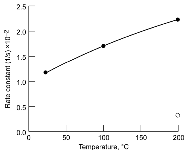
Figure 24.—TiO 2 nanowire sensor response rate versus temperature, filled circles are with Pt catalyst, nonfilled circles are without catalyst.
