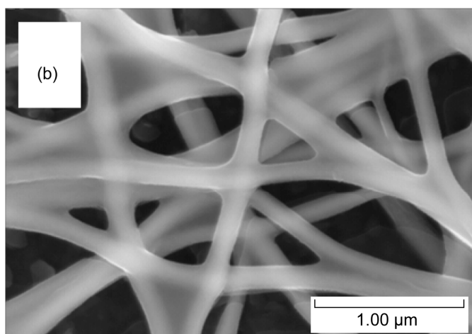
Figure 10.—SEM image of noncalcined SnO 2 nanofibers.
