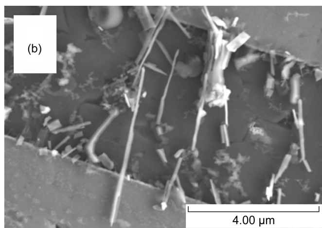
Figure 13.—SEM image of (a) varied morphologies produced by harvesting nanowires grown by controlled oxidation. (b) Their unsuitability to bridge opposing electrodes is apparent.
