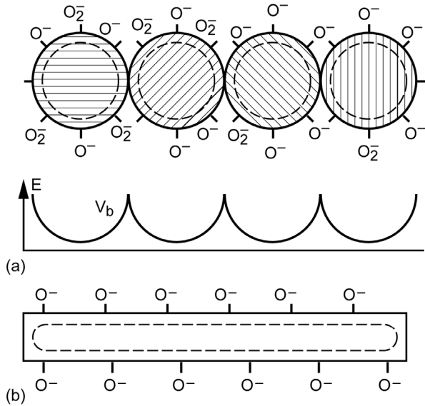
Figure 1.—Schematic illustration of (a) potential barriers between nanoparticles formed by the juxtaposition of depletion layers within a polycrystalline nanofiber and (b) the continuous depletion layer surrounding the nanowire.
