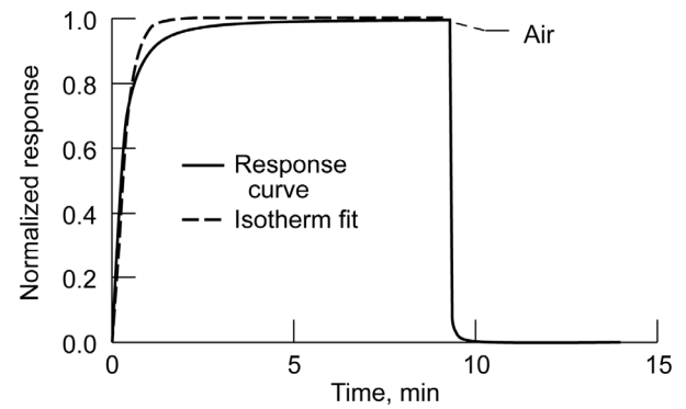
Figure 20.—Isotherm fit on normalized current of a Pd-coated \text{SnO}_2 sensor to 0.5% \text{H}_2 .
