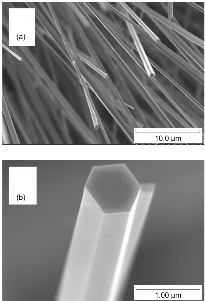
Figure 6.—SEM image. (a) A single-crystal ZnO nanowire, lower resolution. (b) A single-crystal ZnO nanowire, higher resolution.
