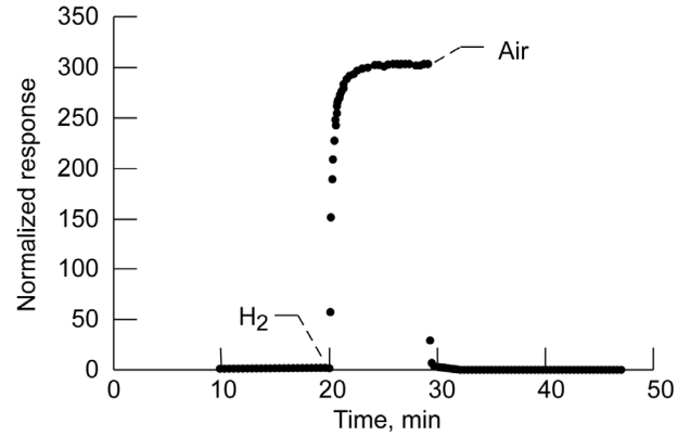
Figure 19.—Normalized response of a Pd-coated \text{SnO}_2 sensor to 0.5% \text{H}_2 .
