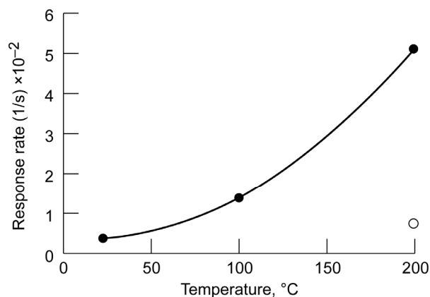
Figure 22.—SnO 2 nanowire sensor response rate versus temperature, filled circles are with Pd catalyst, nonfilled circles are without catalyst.
