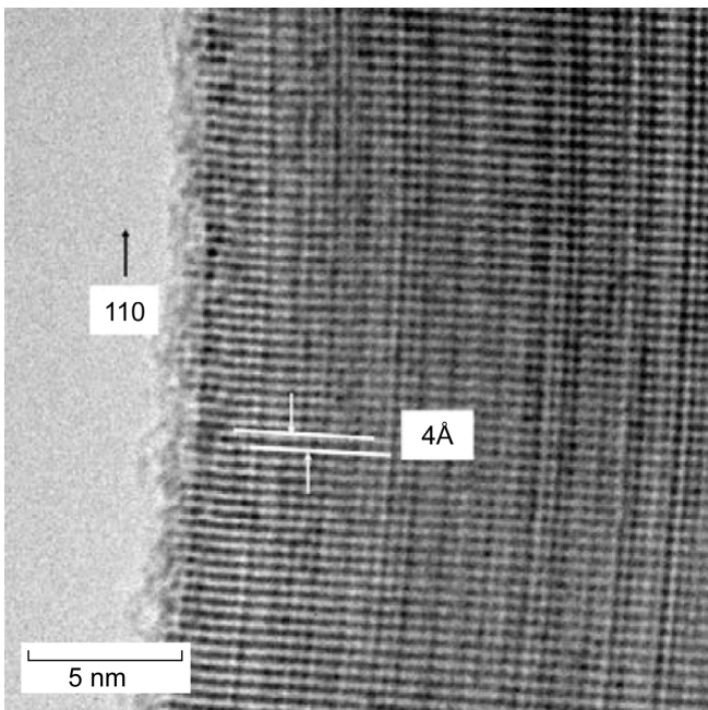
Figure 8.—HTREM image of a TiO 2 nanowire.
