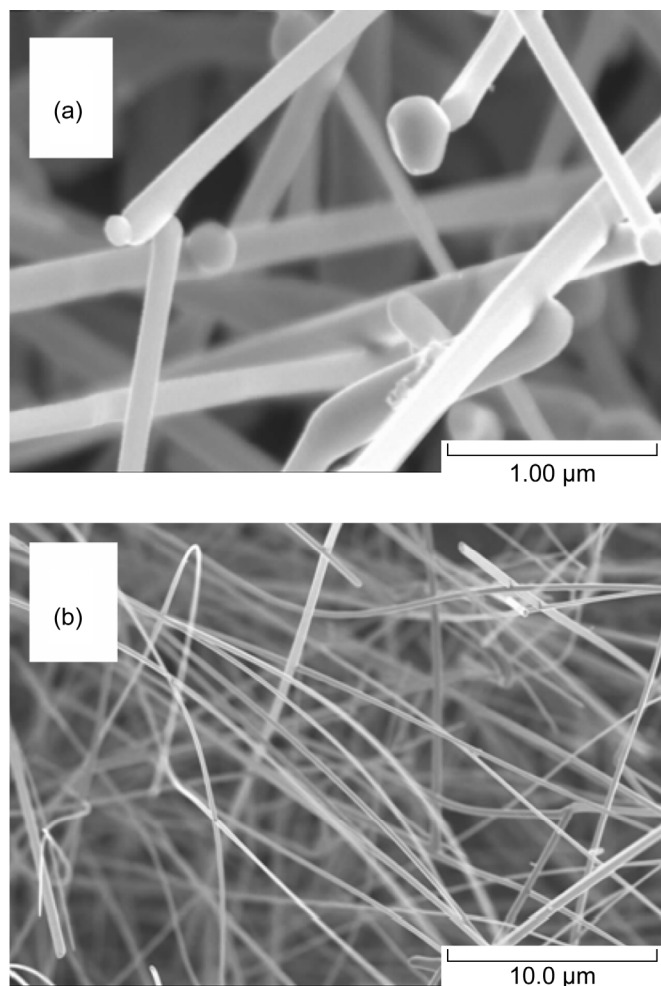
Figure 4.—SEM image of (a) a single-crystal \text{SnO}_2 nanowire, VLS mechanism. (b) A single-crystal \text{SnO}_2 nanowire, versus mechanism.
