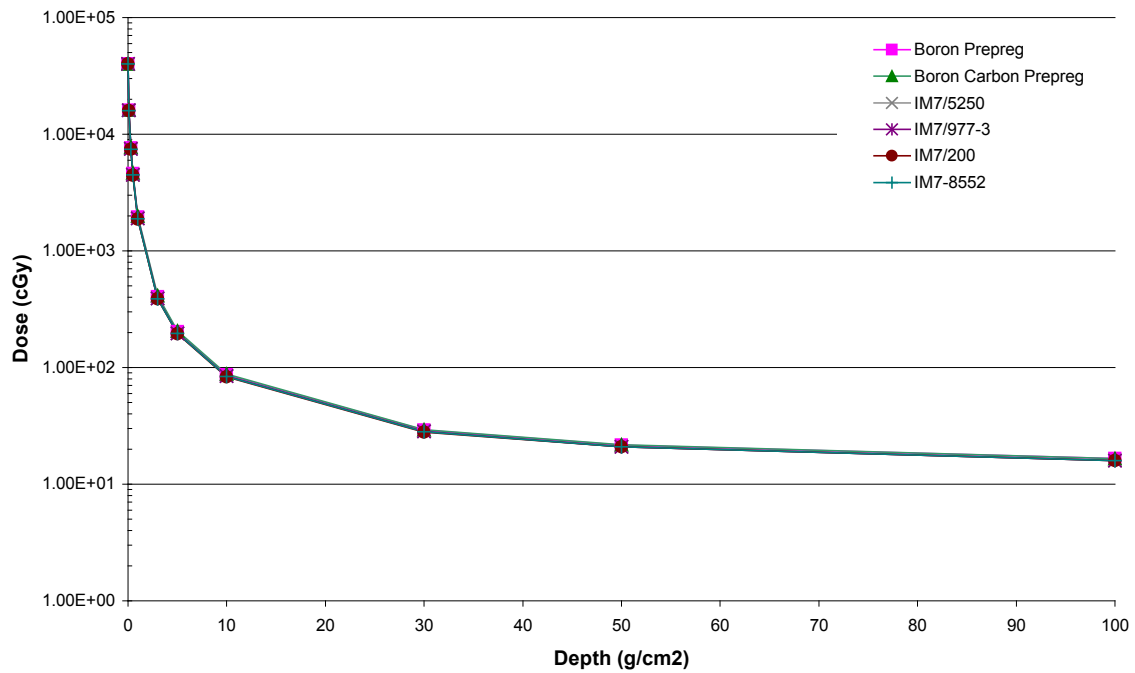
Figure 4: Radiation mitigation properties of boron and carbon fiber composites systems.
