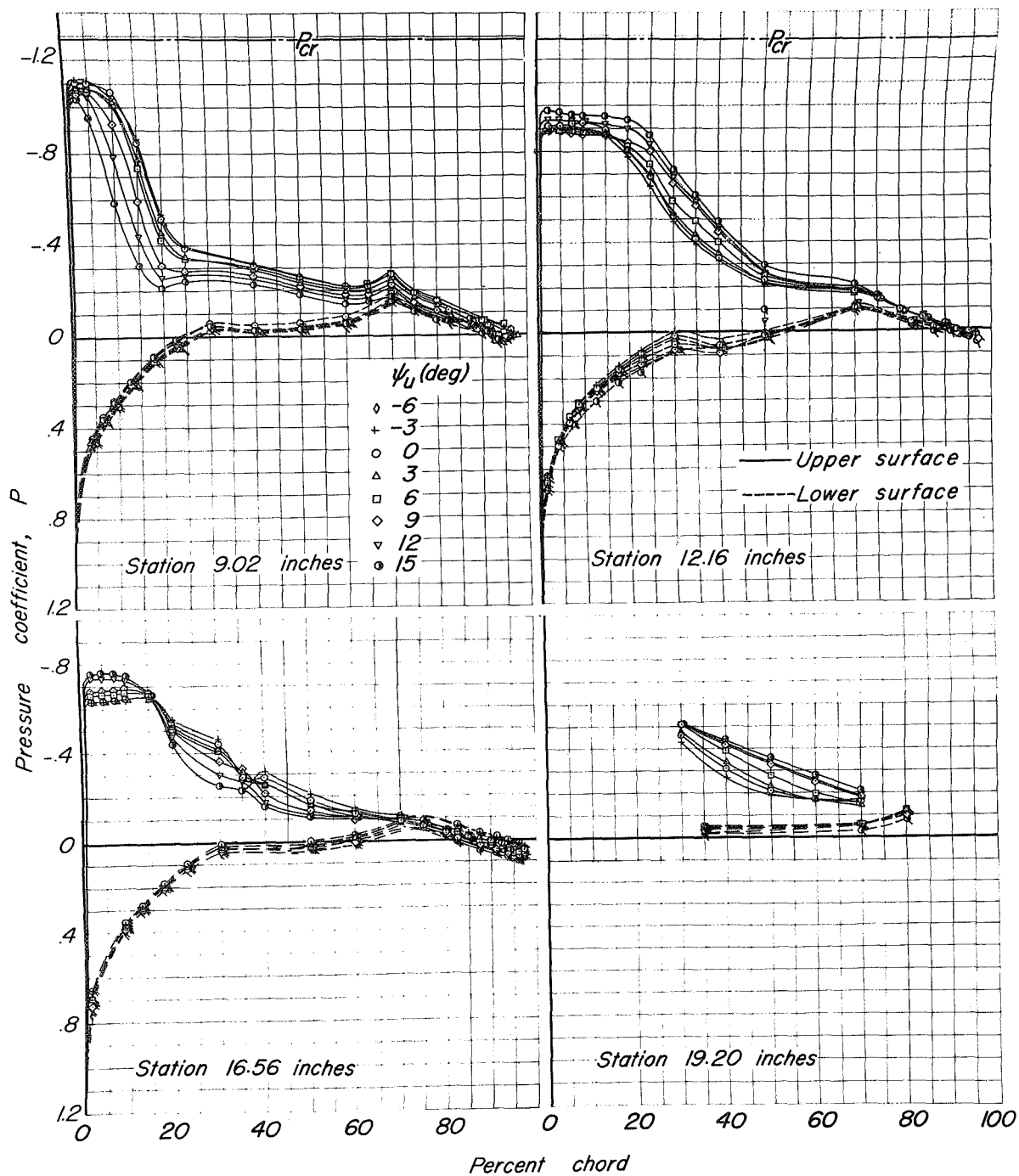
(b) Mach number, 0.60.
