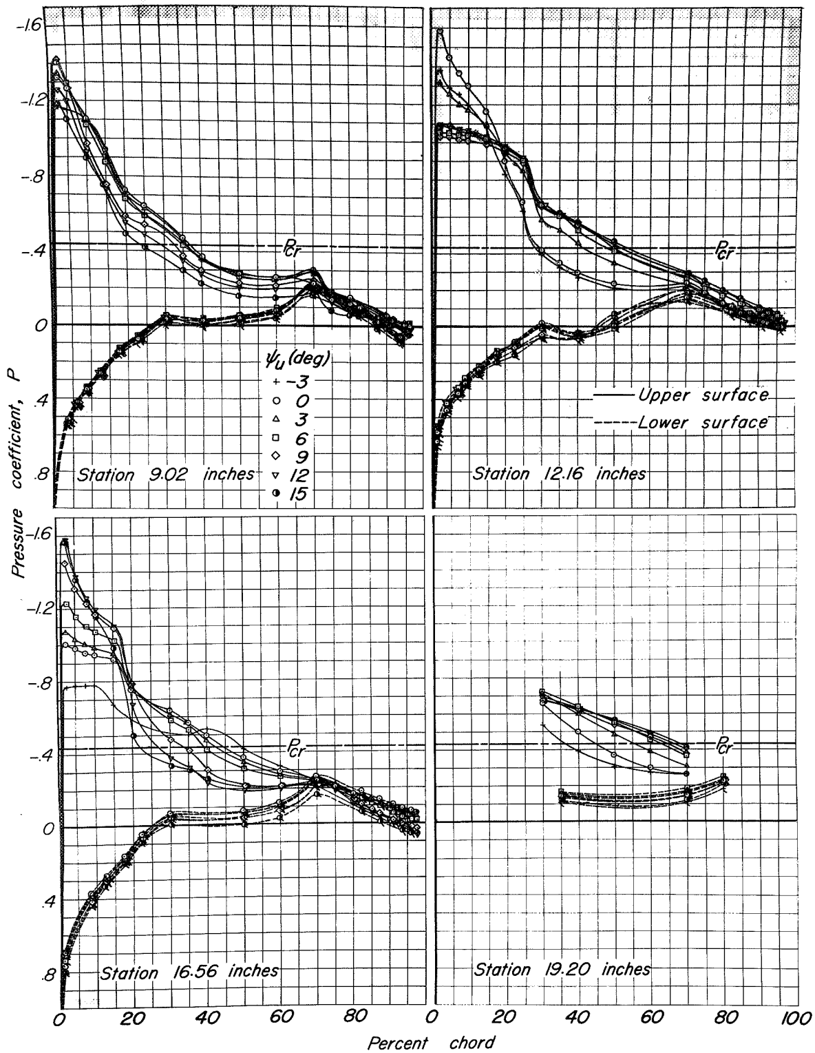
(c) Mach number 0.80.
