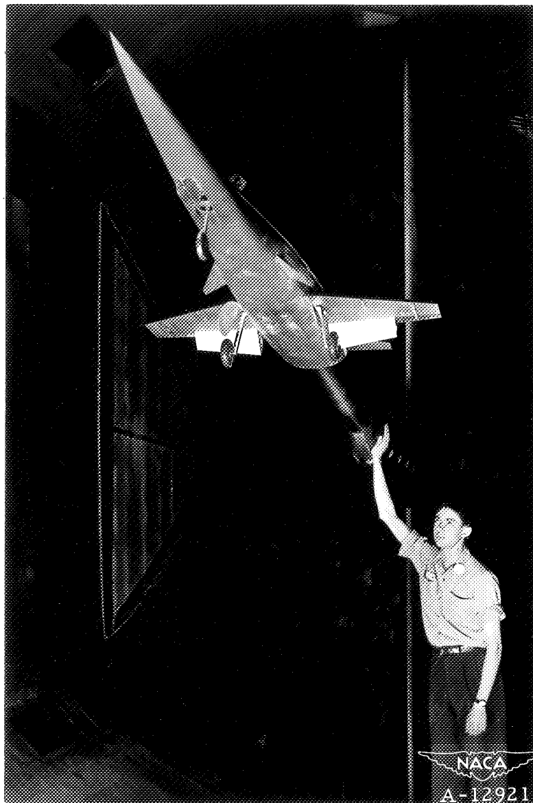
Figure 2.— A three-quarter front view of the MX-656 model with the landing gear extended, the flaps deflected, and the nose fins in the normal position.
