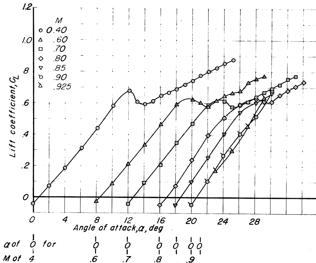
(a) Lift characteristics.
