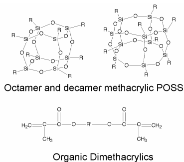
Figure 2b: MA8000 structure
