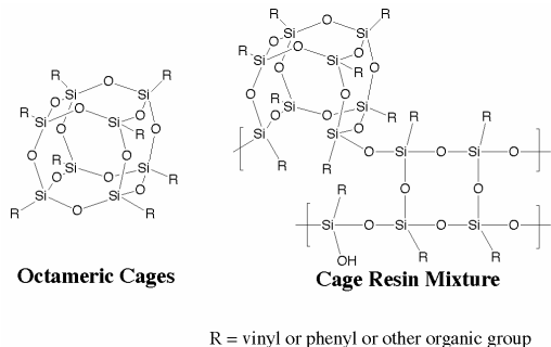
Figure 2a: PM1287 structure
