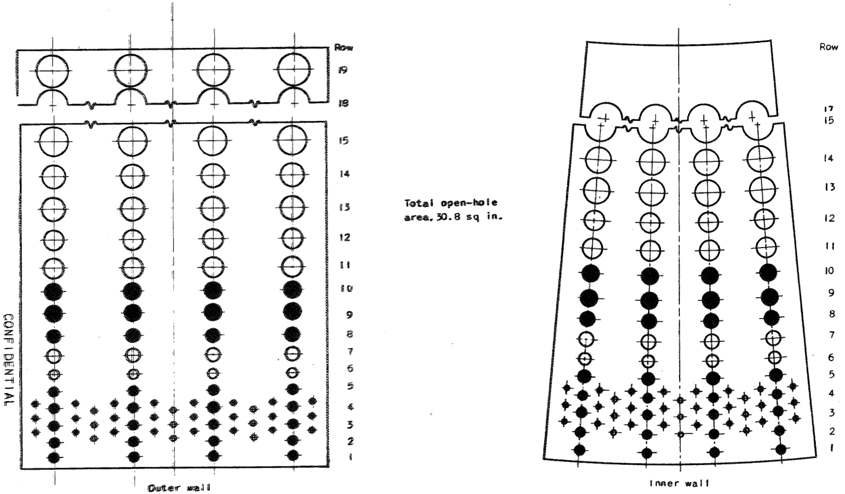
(b) Modification I (shaded holes blocked).
