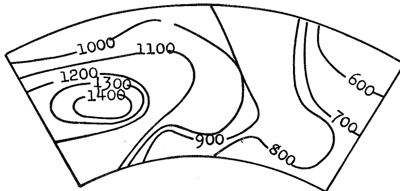
(b) Modification 1. Average combustor-outlet temperature, 952^{\circ} F.
