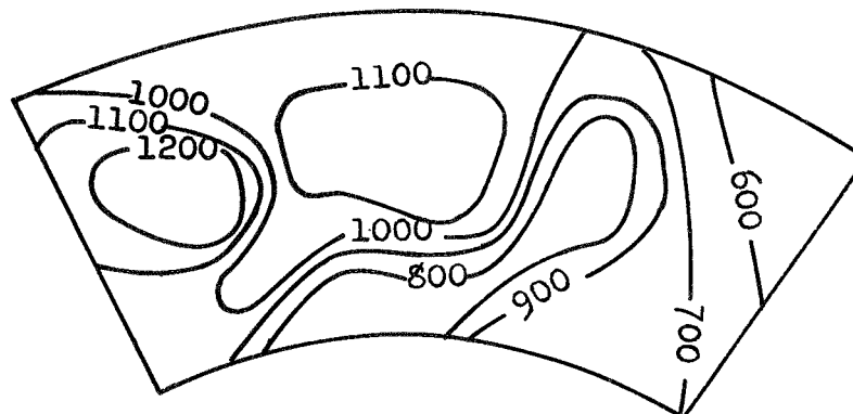
(c) Modification 2. Average combustor-outlet temperature, 960^{\circ} F.
