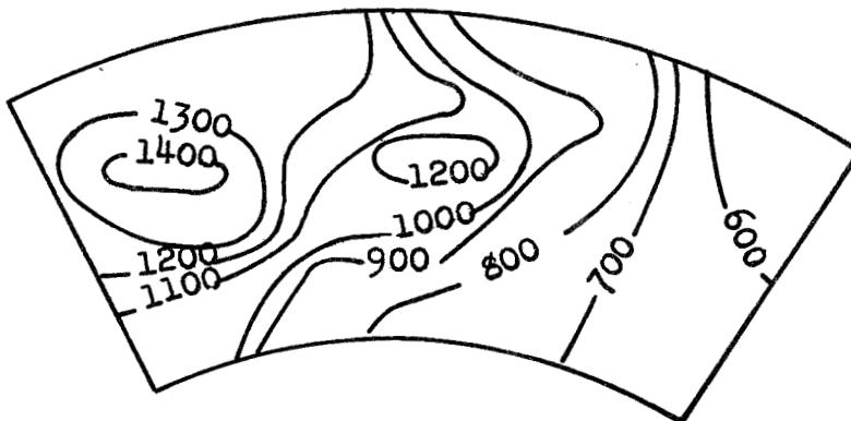
(e) Modification 4. Average combustor-outlet temperature, 969° F.
