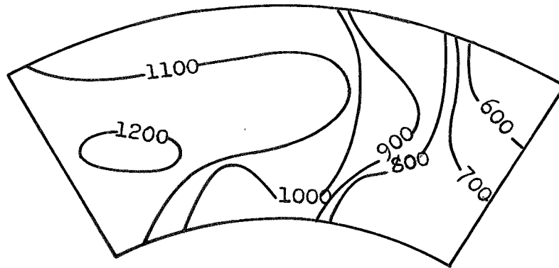
(a) Original design. Average combustor-outlet temperature, 970^{\circ} F.
