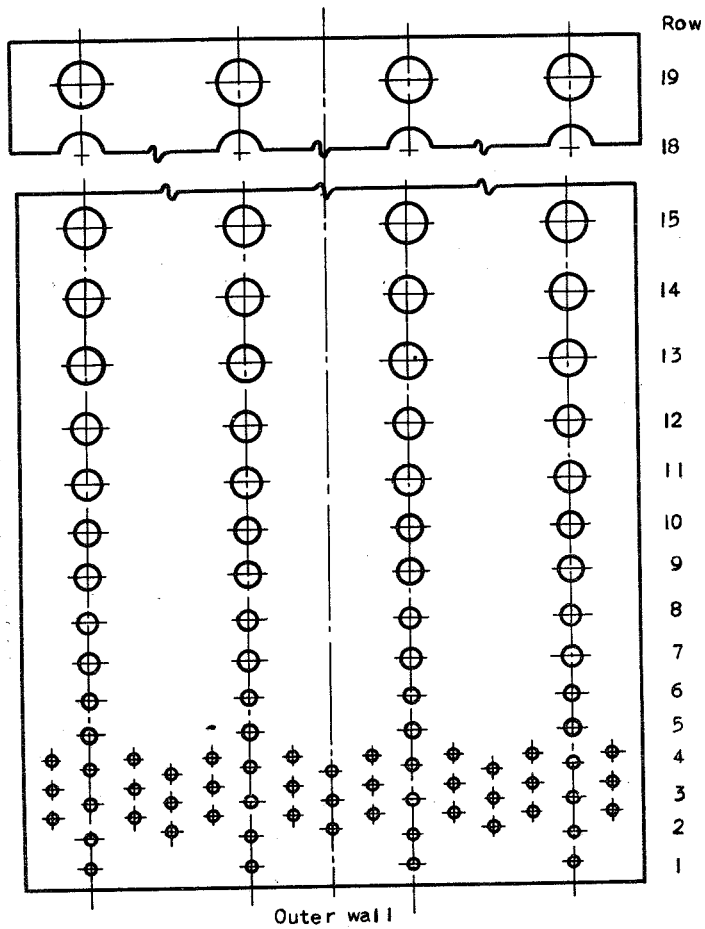
Figure 5. - Continued. Development of basket walls of one-sixth combustor segment.
