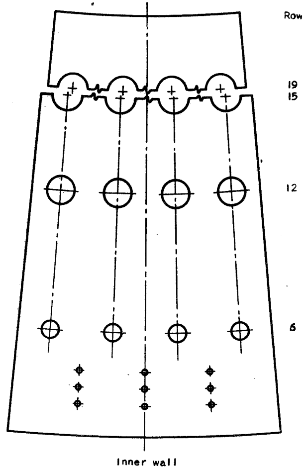
Figure 5. - Concluded. Development of basket walls of one-sixth combustor segment.
