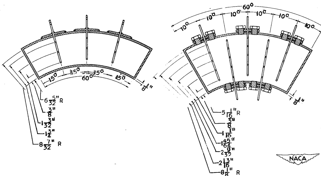
(c) Inlet total-pressure rakes, downstream at station 1.
