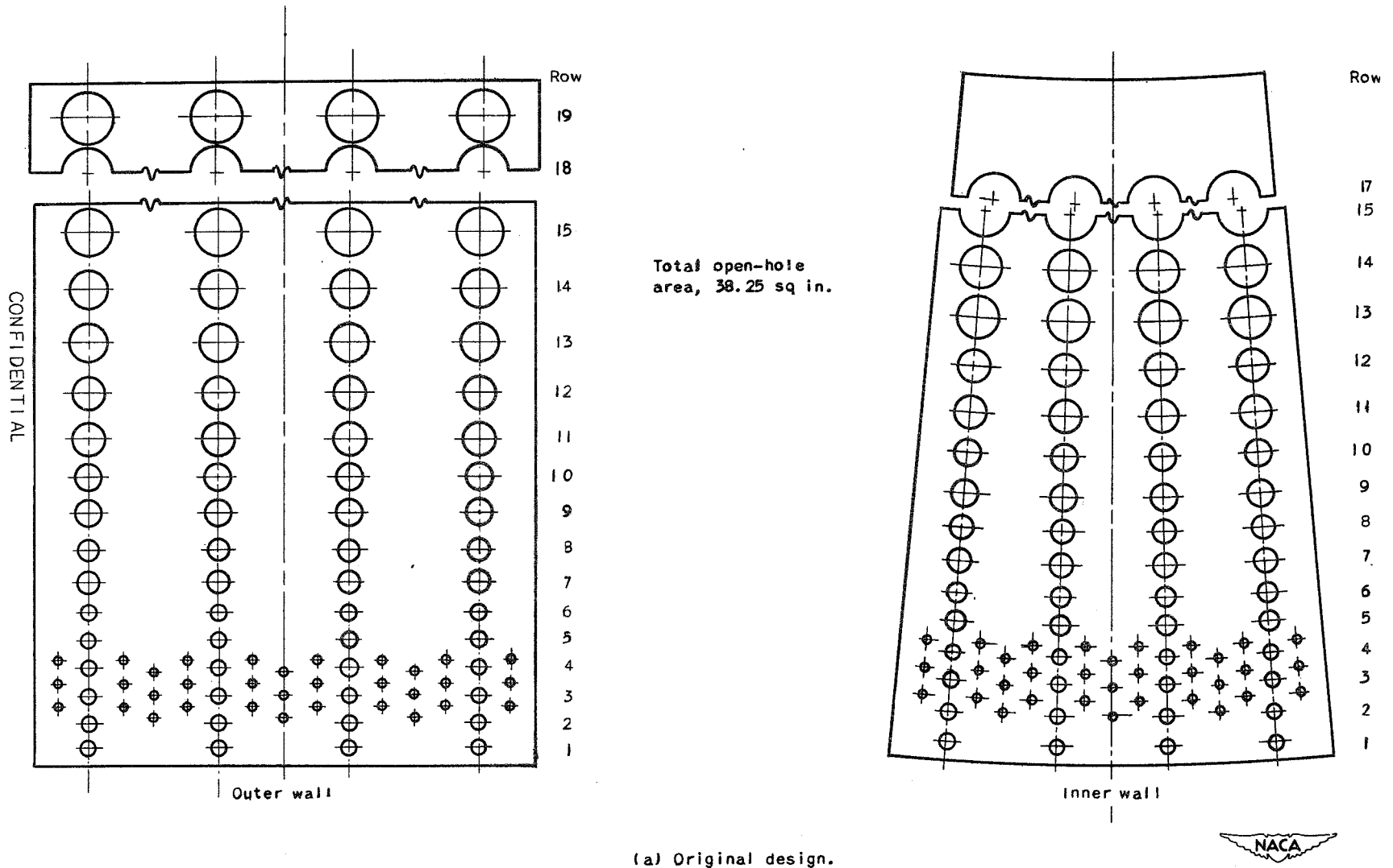
Figure 5. - Development of basket walls of one-sixth combustor segment.
