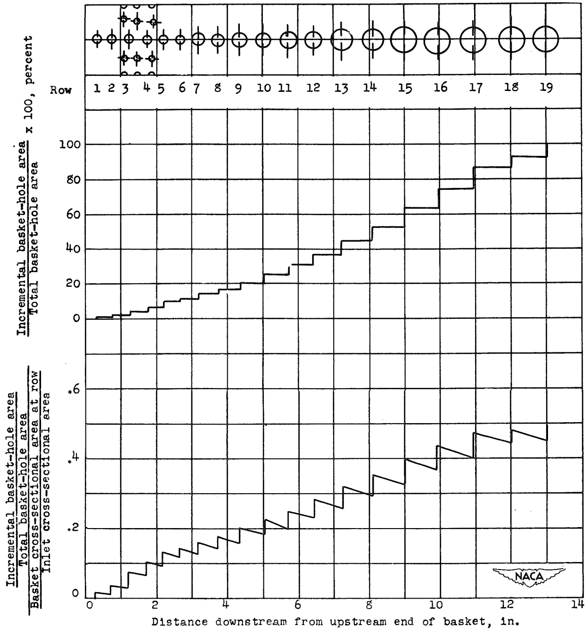
(a) Original design.
