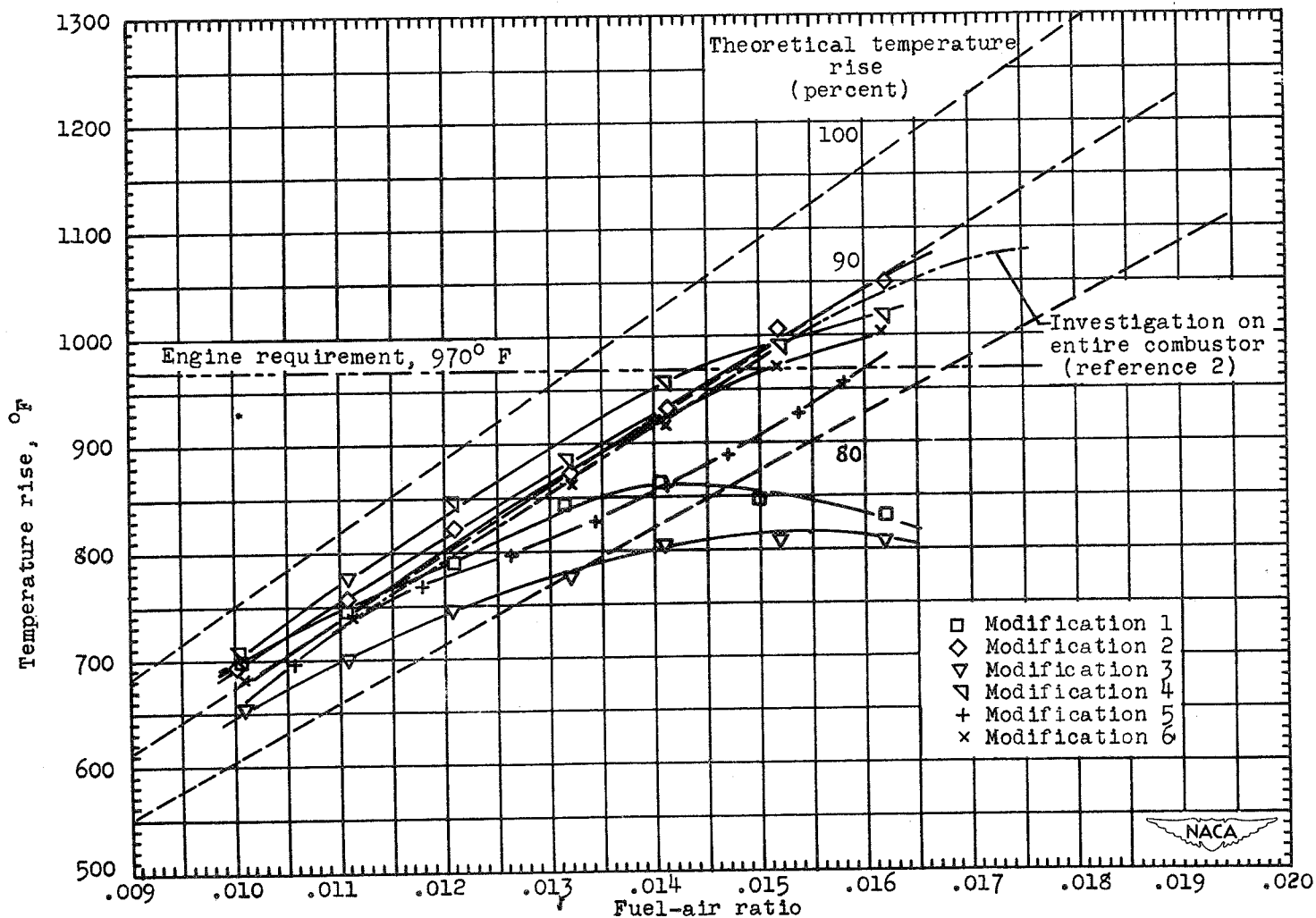
(d) Operating conditions for 19B engine at altitude of 30,000 feet and engine speed of 16,500 rpm: air flow, 1.87 pounds per second; inlet-air total pressure, 16.0 pounds per square inch absolute; inlet-air temperature, 190° F.
