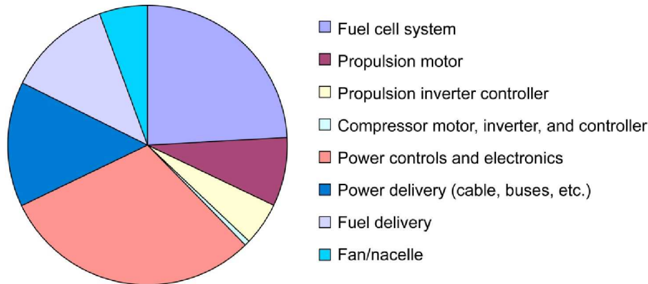
Figure 7.—Initial relative masses of hydrogen fuel cell propulsion system components.
