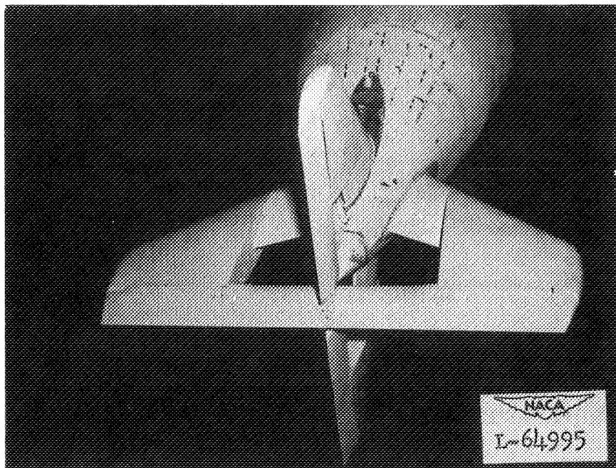
Figure 2.- Scheme-2 fin and rudder with 332-square-foot diving planes installed.
