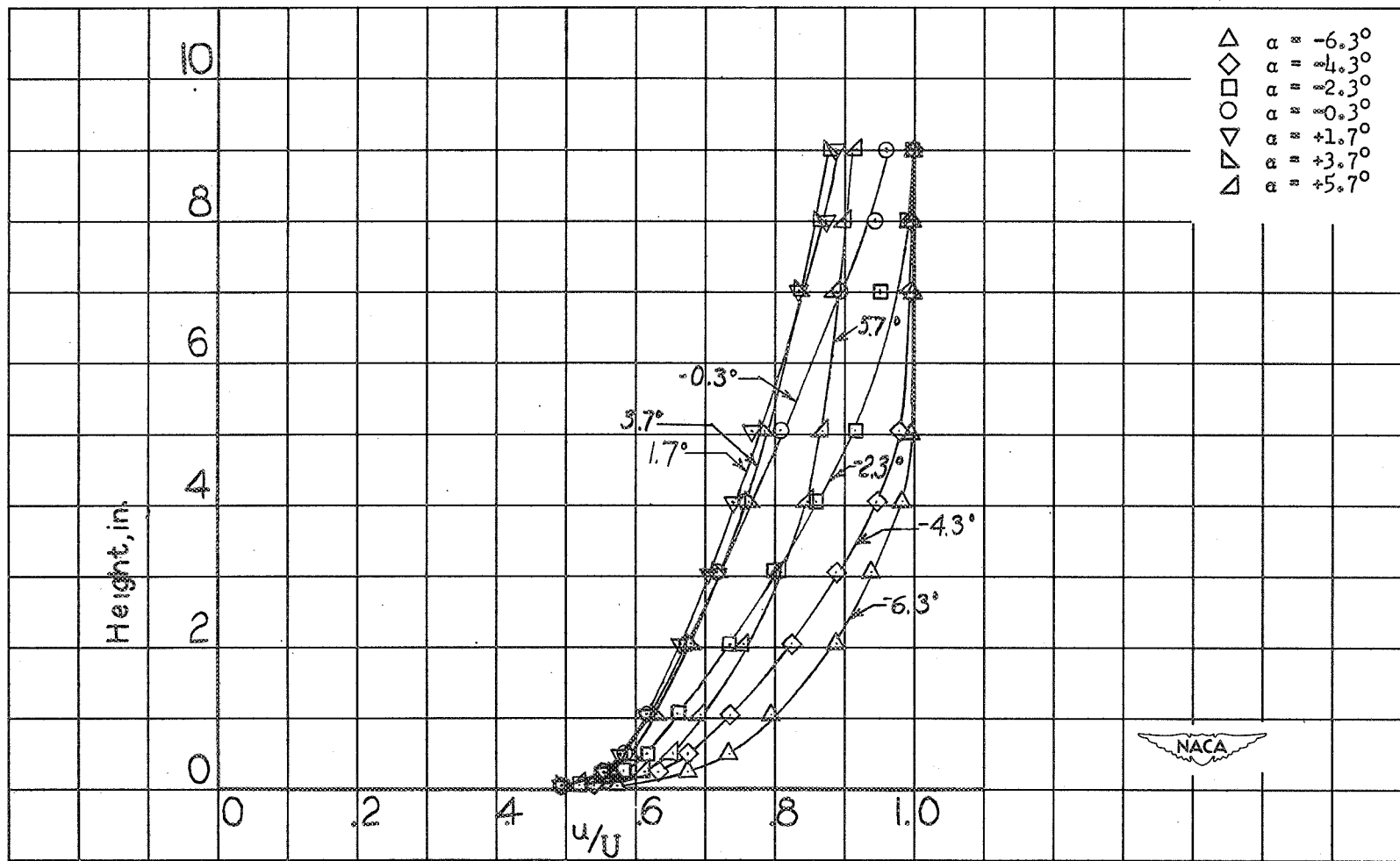
(b) Effect of angle of attack. Position, 0.96l.
