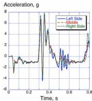
(b) Seat platform accelerations.
