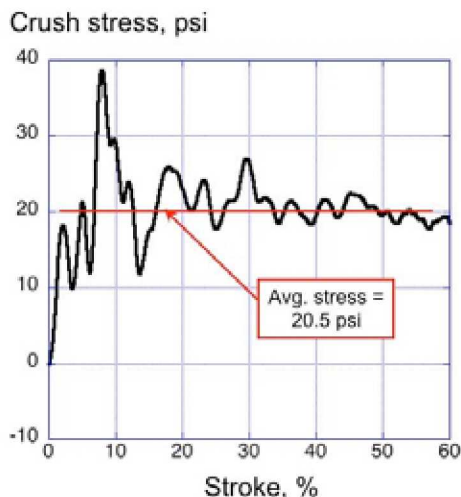
(a) Dynamic crush response.
