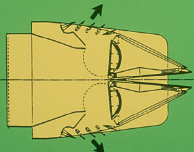
Rotating Vane Vectoring
