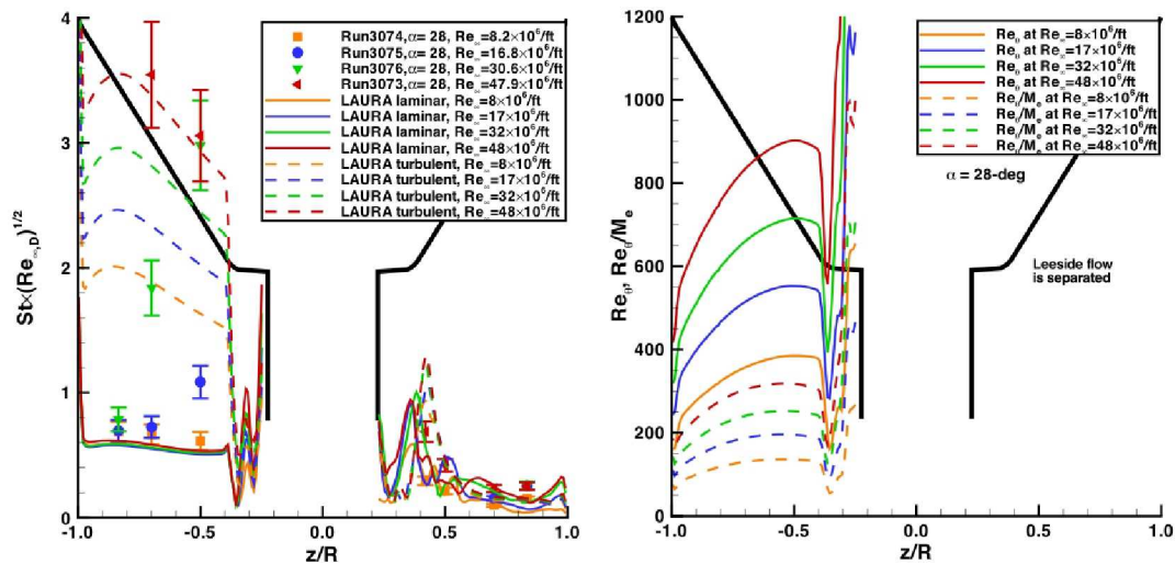
Figure 16. Aftbody Heating and Boundary-Layer Parameters, AEDC Tunnel 9, Mach 8 nozzle, \alpha = 28\text{-deg}
