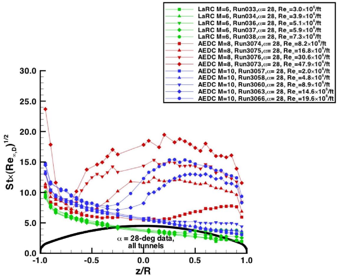
Figure 17. \alpha = 28 -deg distributions using total enthalpy
