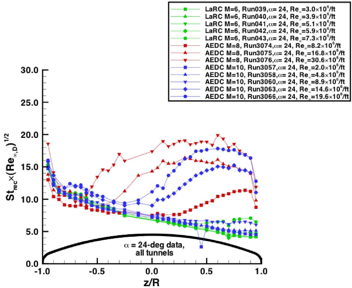
Figure 19. \alpha = 24\text{-deg} distributions using adiabatic wall enthalpy
