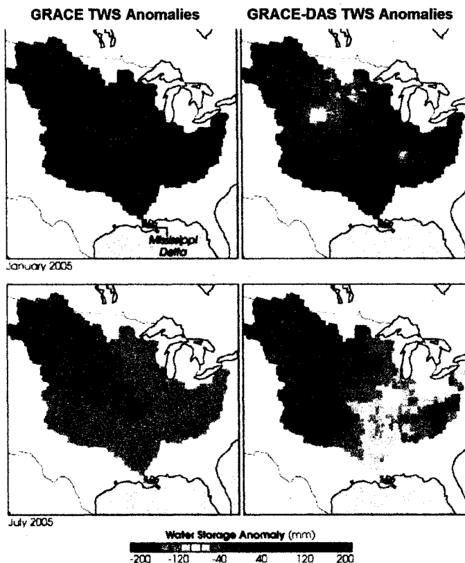
Figure 2. GRACE provides terrestrial water storage anomalies for large regions, such as river basins (left). The GRACE data assimilation system, based on the Catchment land surface model, synthesizes the GRACE data and produces high resolution output (right).
