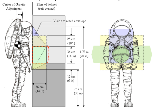
Figure 10 Lunar EVA Work Envelope
