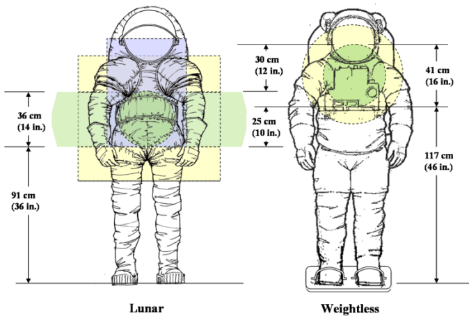
Figure 12 Lunar and Weightless Envelopes
