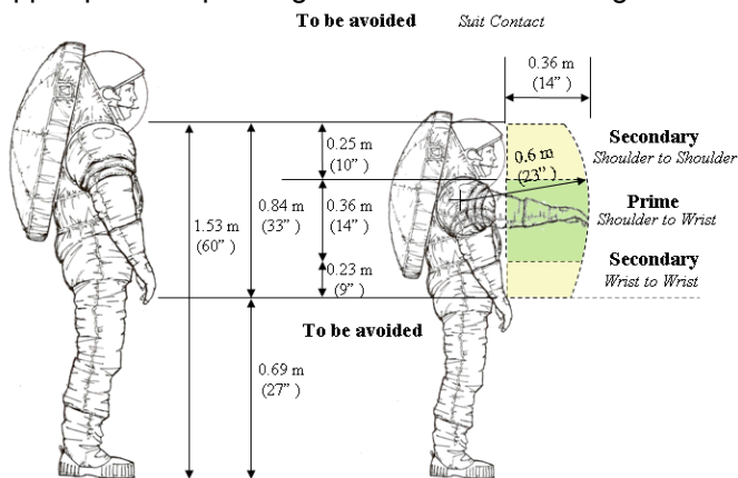
Figure 8 Primary and Secondary Reach Envelopes
