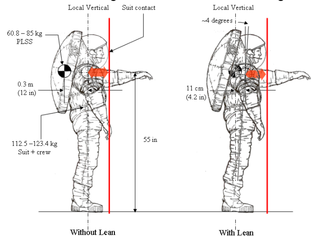
Figure 7 Static Lean and Reach Envelope
