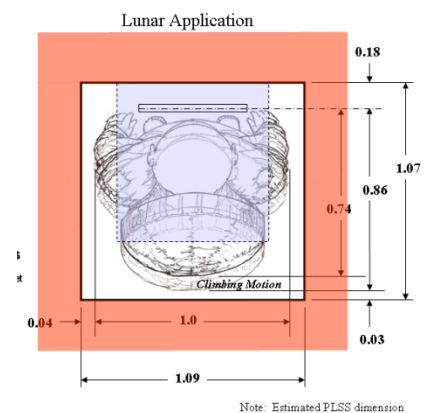
Figure 14 Vertical Translation Corridor
