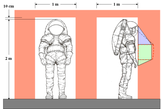
Figure 13 Horizontal Translation Corridor
