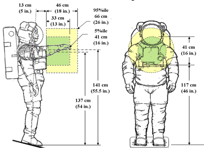
Figure 1 Weightless EVA Work Envelope
