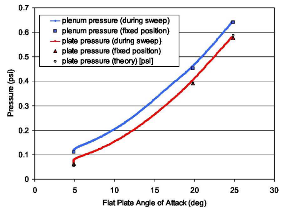
Figure 8 Pressure in the NO seeding chamber ( plenum pressure ) and on the surface of the flat plate ( plate pressure ) during an angle of attack sweep for a P_0 = 720 psi run with an NO flowrate of 0.3 slpm.
