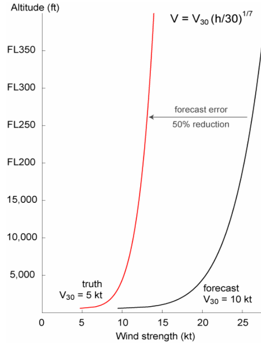
Figure 2: Plot of Truth and Forecast Winds and Wind Forecast Field
