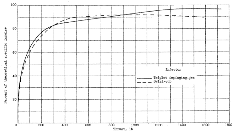
Figure 24. Theoretical Specific Impulse for Triplet Impinging-Jet Variable Area Injector
