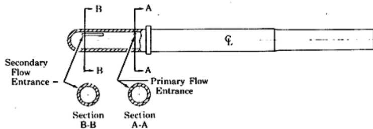
Figure 13. XLR-129 Dual-Inlet Swirl Coax Oxidizer Element
