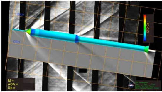
Figure 8. Combination of experimental Schlieren photograph with computational prediction of flow density as well as surface pressure distribution on Ares rocket.
