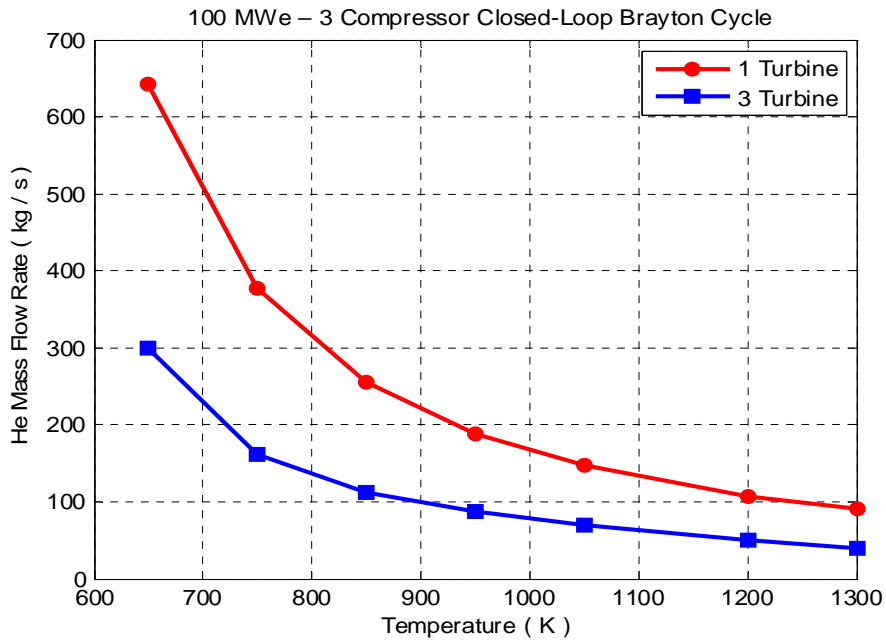
Figure 7.—Power plant mass flowrate as a function of turbine inlet temperature for only intercooled (one turbine) and intercooled + reheated (three turbines)—100 MWe CCGT power plant.
