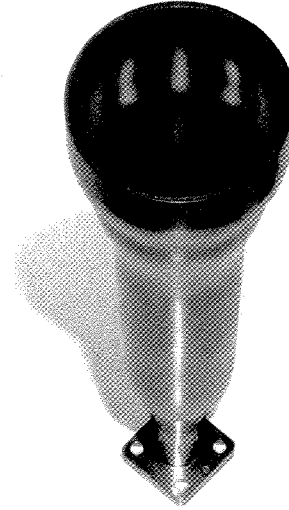
Fig. 3. A smooth-walled feedhorn operating between 33 and 45 GHz was constructed. The horn is 140 mm long with an aperture radius of 22 mm. The input circular waveguide radius is 3.334 mm.
