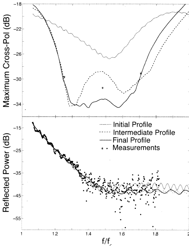
Fig. 2. (Top) The maximum cross-polar response across the band is shown for the three profiles in Figure 1. Measurements of the maximum cross-polarization are superposed. (Bottom) The reflected power measurements for the final feed horn are shown plotted over the predicted reflected power for the initial, intermediate, and final feedhorn profiles. Frequency is given in units of the cutoff frequency of the input circular waveguide.
