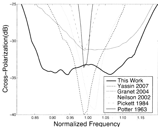
Fig. 5. The maximum cross-polar response of the prototype feedhorn is compared to other implementations of smooth-walled feedhorns. The data presented have been normalized to the design center frequencies as specified by the respective authors.
