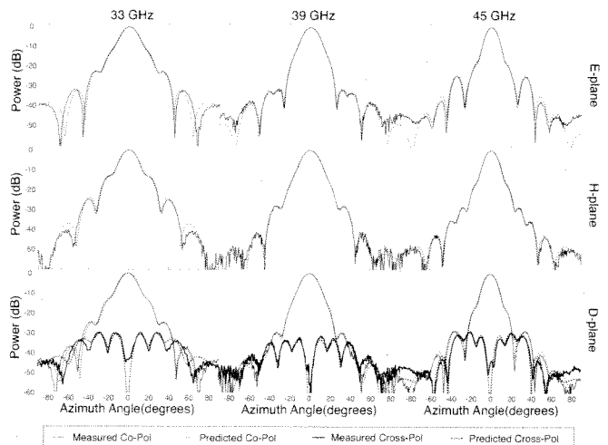
Fig. 4. The measured E -, H -, and diagonal-plane angular responses for the lower edge (33 GHz), center (39 GHz), and upper edge (45 GHz) of the optimization band are shown. The cross-polar patterns in the diagonal plane are shown in the bottom three panels for each of the three frequencies.
