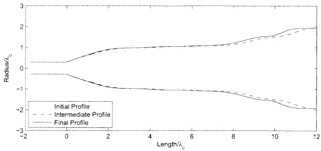
Fig. 1. The initial, intermediate and final profiles are shown. All dimensions are given in units of the cutoff wavelength of the input circular waveguide.
