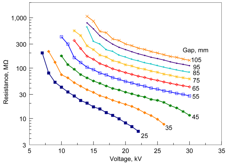
Figure 8.6.—The resistance of the corona discharge as a function of gap and voltage.
