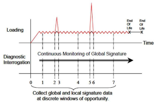
Figure 3.—Temporal interrogation of a given component.
