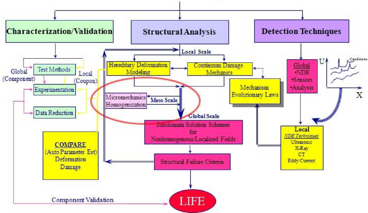
Figure 6.—Multiscale framework describing the interaction between experimentation, analysis and detection techniques to enable accurate deformation and life modeling.
