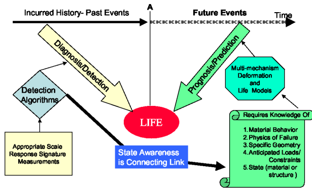
Figure 1.—Depicts the distinction between diagnostic and prognostic methodologies and their integration.
