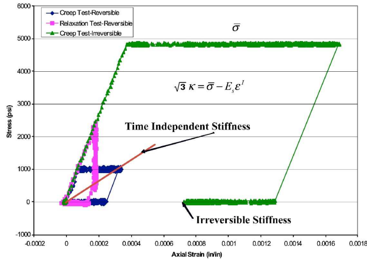
Figure 10.—Determination of threshold stress and time-independent stiffness for GVIPS model.
