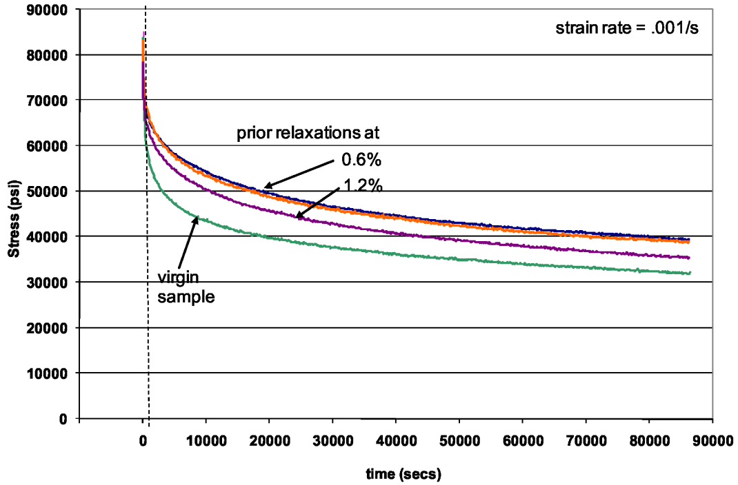
Figure 17.—Stress-time results for relaxation at 1.8 percent strain from relaxation and step relaxation tests conducted at 427 °C to demonstrate history dependence of viscoplastic behavior.
