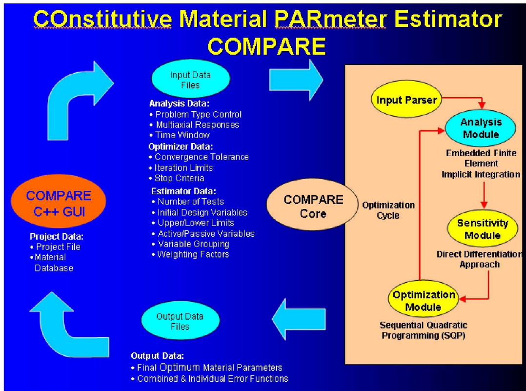
Figure 8.—Flow chart for COMPARE software.
