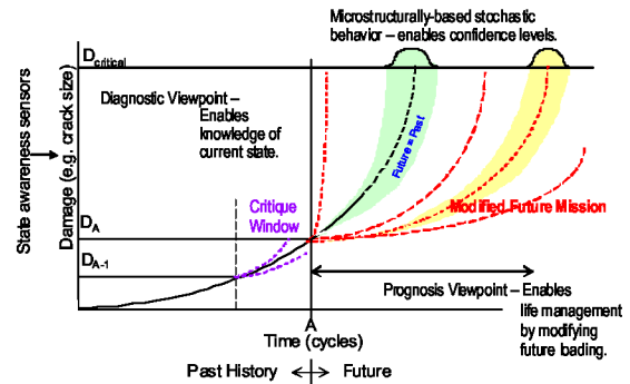
Figure 2.—Depiction of an integrated diagnostic and prognosis approach to incrementally updating a life management system.
