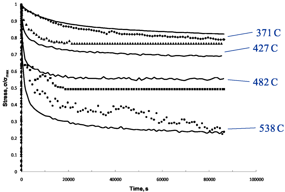
Figure 13.—Correlation of viscoelastic relaxation stress-time response at various temperatures for Ti-6-4.
