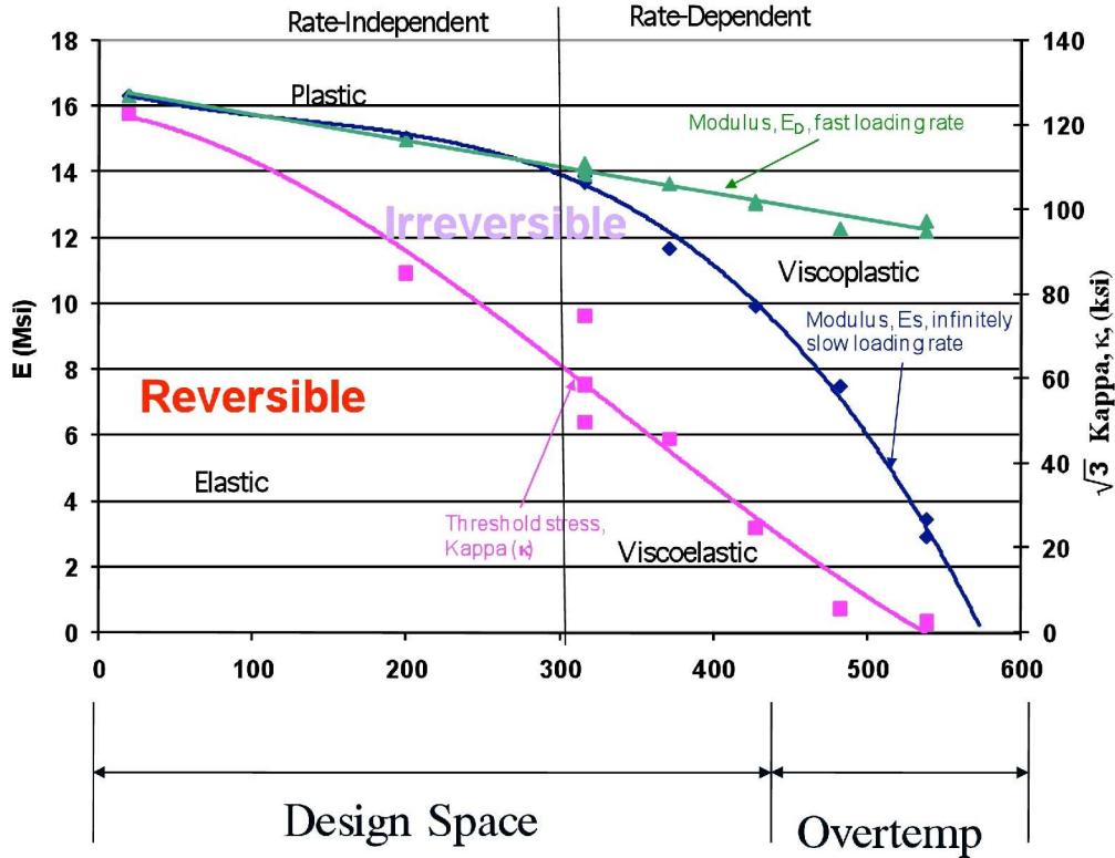
Figure 9.—Variation of modulus and threshold stress as a function of temperature for Ti-6-4 material.
