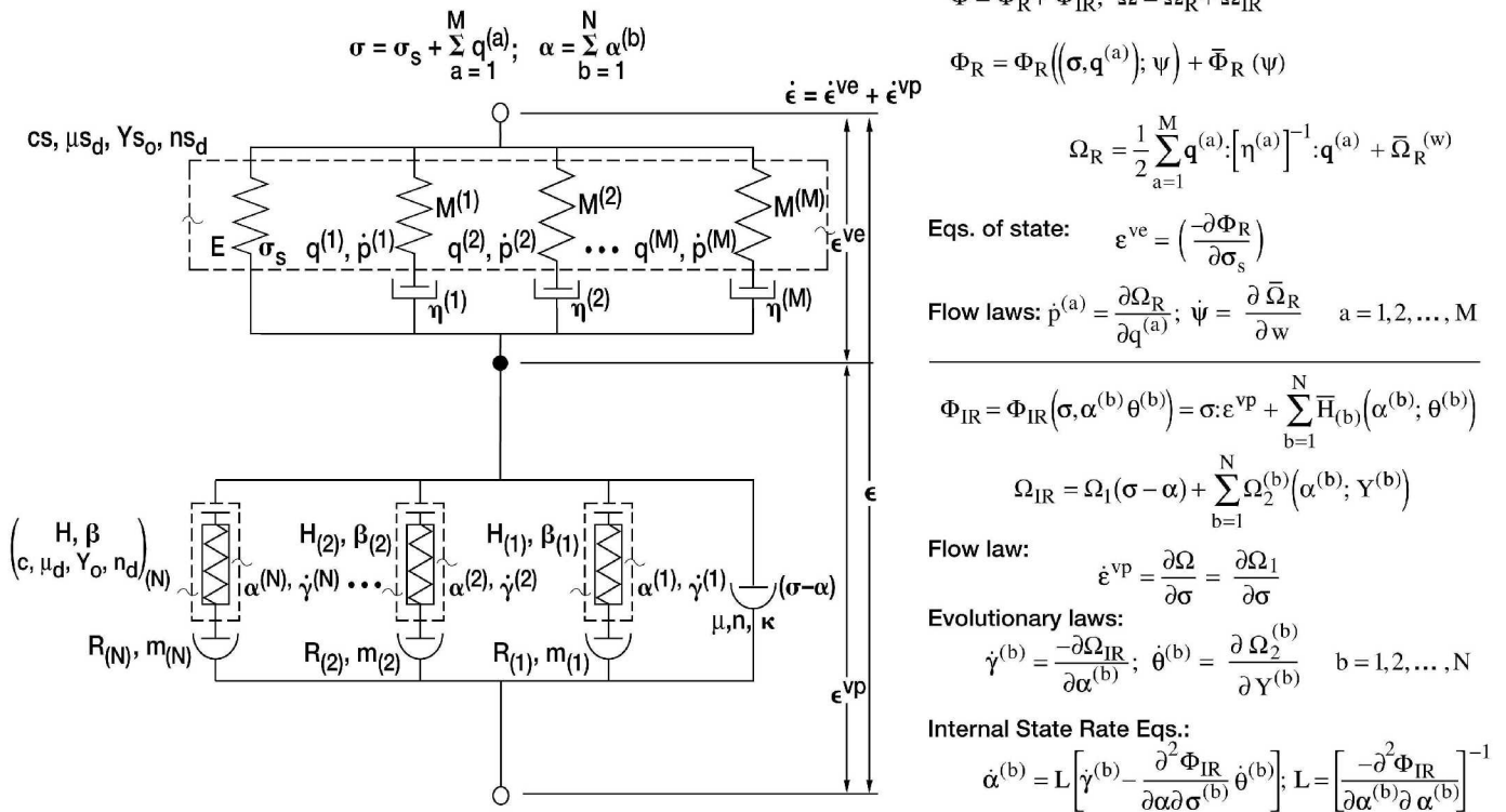
Figure 7.—Analog representation of multimechanism deformation and damage GVIPS framework with key governing equations.
