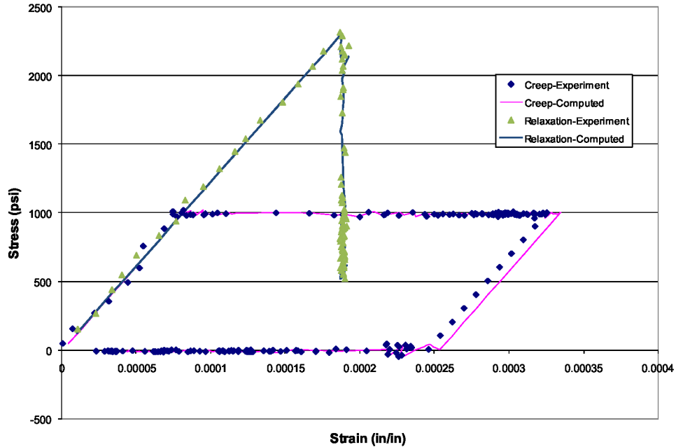
Figure 12.—Correlation of viscoelastic creep and relaxation response of Ti-6-4 at 538 °C.
