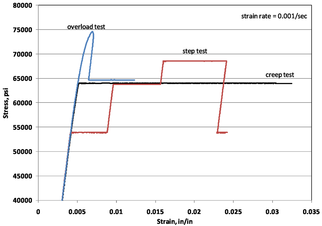
Figure 18.—Stress-strain curves of creep, step creep and creep overload tests at 427 °C.
