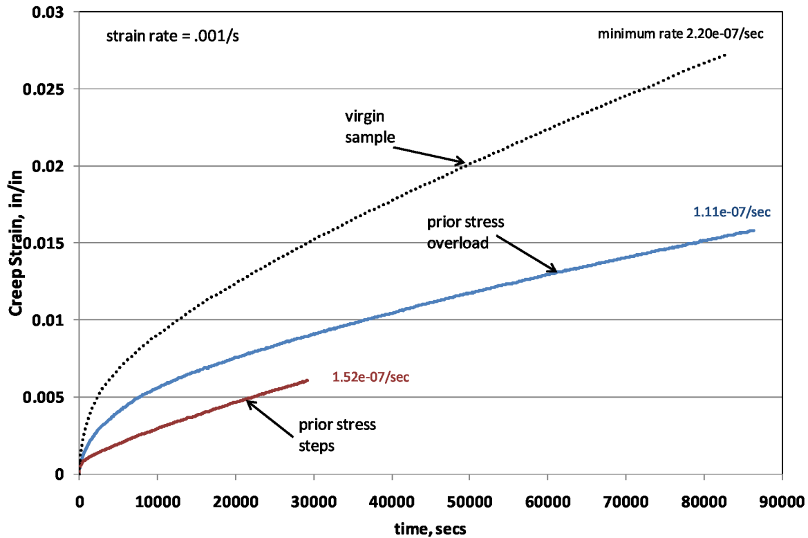
Figure 19.—Strain versus time results from creep tests conducted at 65 ksi and 427 °C to demonstrate history dependence of viscoplastic material behavior.
