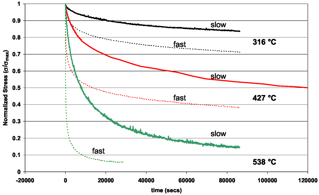
Figure 15.—Effect of strain rate and temperature on viscoplastic relaxation response for Ti-6-4 material.
