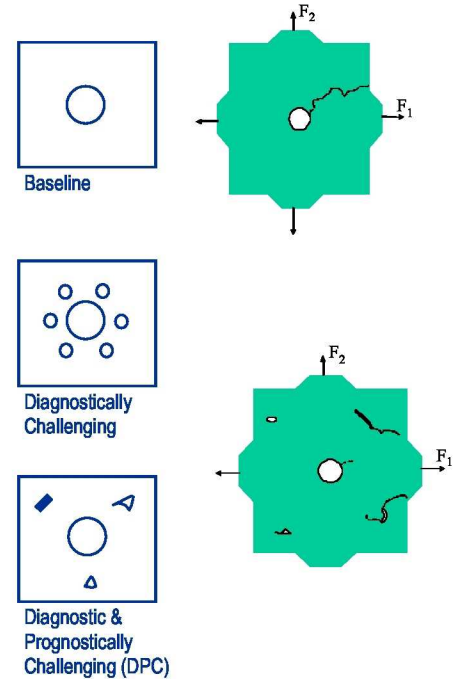
Figure 4.—Schematic of biaxially loaded plate with various inflicted defect configurations.
