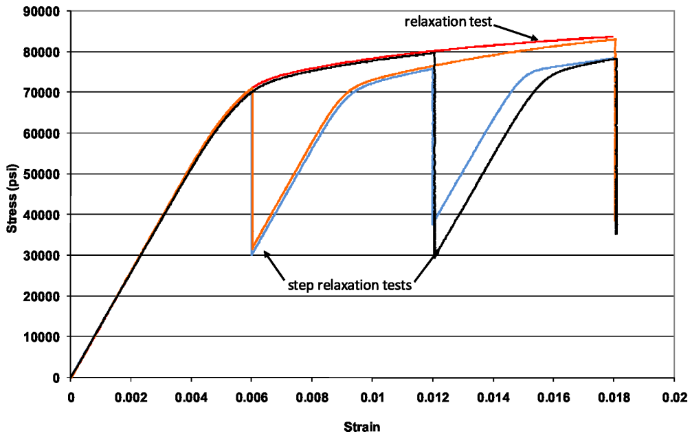
Figure 16.—Stress-strain results from relaxation and step relaxation tests conducted at 427 °C to demonstrate history dependence of viscoplastic behavior.
