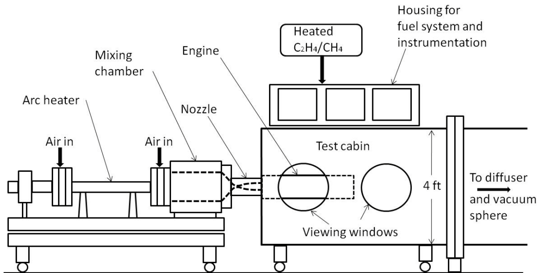
Figure 4. Facility schematic.
