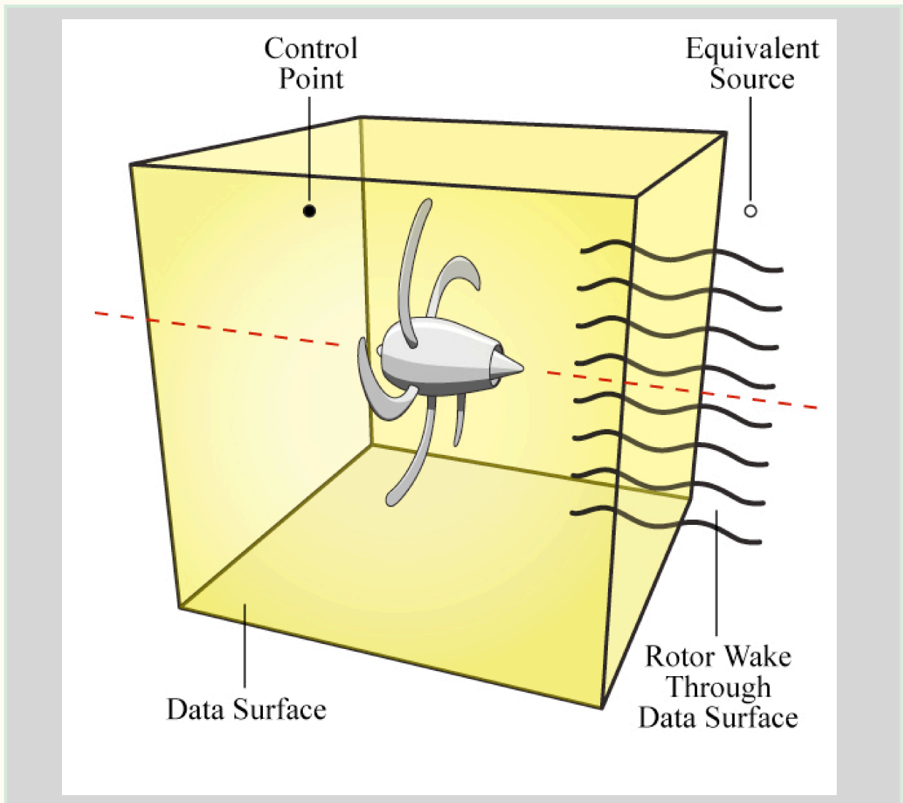
Figure 3- Sketch of the data surface for FW – H_{pds} code and the use of equivalent sources to generate the null field inside the data surface at control points. Here we show one equivalent source and one control point for simplicity.
