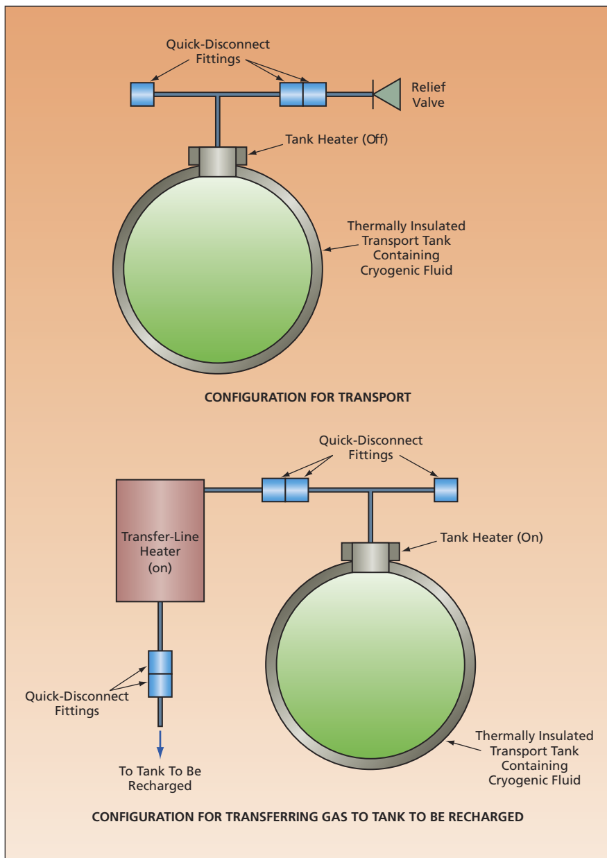
An Insulated Transport Tank would contain a cryogenic fluid, which would be warmed to convert it to a pressurized gas.
