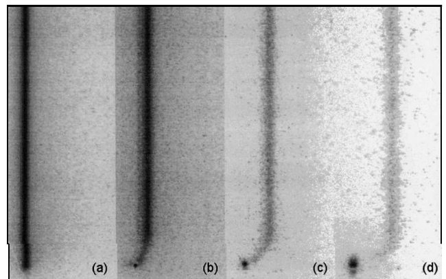
Fig. 5 Raw LIF intensities for four delays: 0, 250, 500, and 750 ns for a–d, respectively. Image a was obtained in static \text{NO} in the test section. Images b–d were obtained during the shock-tunnel flow.
