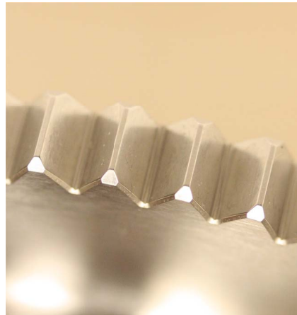
Figure 5.—Photograph of HPA gears before testing.
