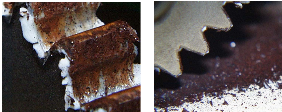
Figure 8.—Left: shows rust forming on the gear profile. Right: shows rust debris from metal on metal contact. (Both photos from a 2.12 module (12-diametral pitch) gear test.)
